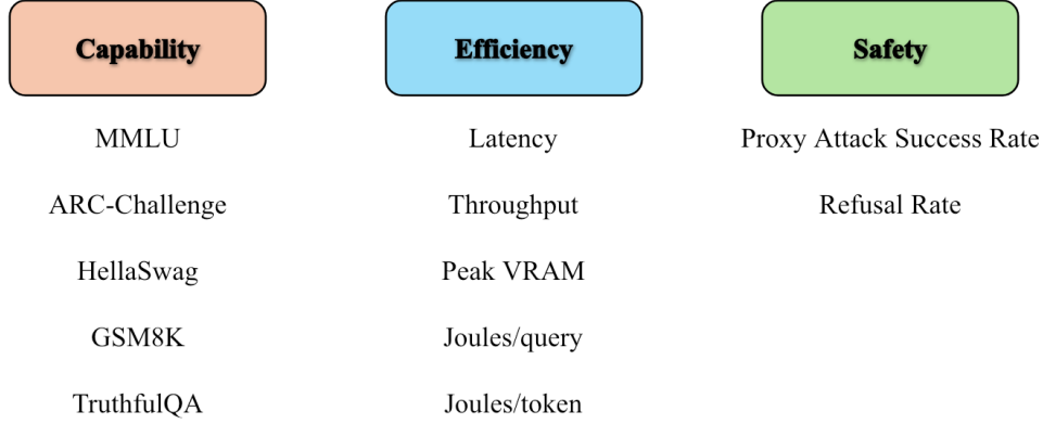
Figure 2: Measured metrics. Capability, systems efficiency, operational energy and refusal behavior are retained separately before aggregation.
