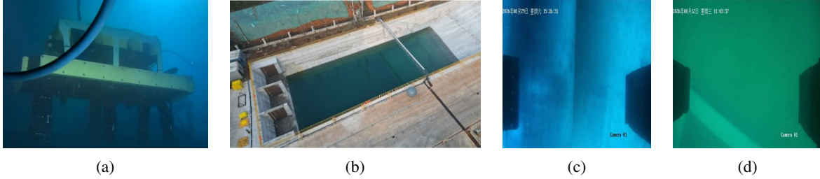
Fig. 9. Field experimental conditions. (a) The heavy-duty underwater salvage ROV used in this study. (b) The test pool: 60 m by 20 m, 10 m deep. (c) The aluminum pipe on the pool floor. (d) The steel frame on the pool floor.
