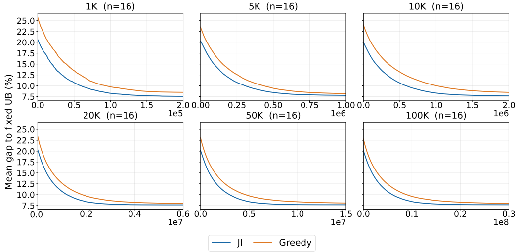
Figure 5: GAP convergence trajectories during 2-opt refinement with greedy and JI initializations across six TSP scales.
