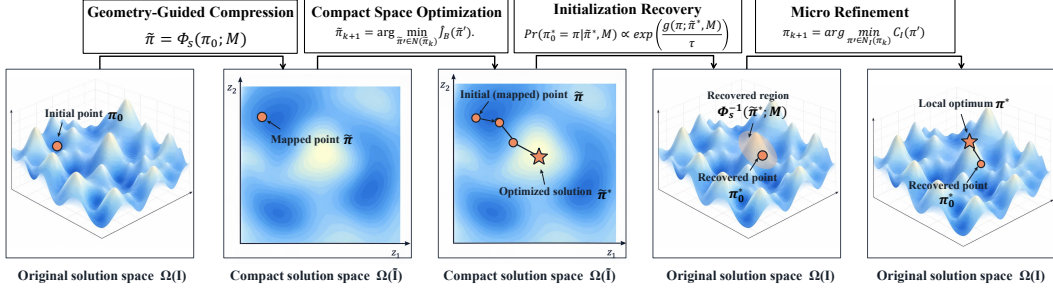
Figure 2: Overview of Just Initialize. The framework compresses the original solution space, optimizes in a compact space, recovers an optimization-friendly initialization, and performs lightweight refinement in the original space.
