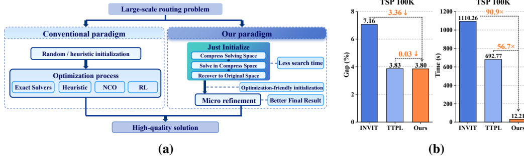
Figure 1: Rethinking large-scale routing optimization. (a) Conventional paradigm and our paradigm. (b) Performance comparison with SOTA methods on 100K-node TSP instances.
