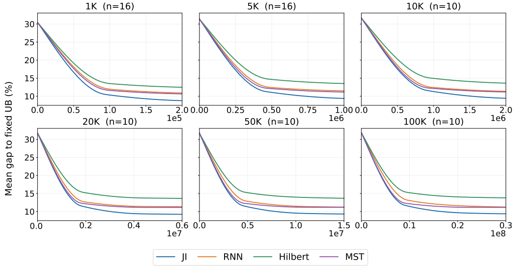
Figure 4: GAP convergence trajectories during 2-opt refinement under matched initializations across six TSP scales.
