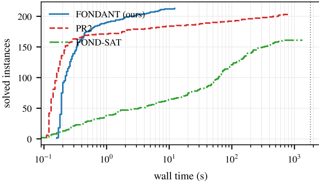
Figure 1: Solved instances versus wall time (log scale), FONDANT (ours, solid), PR2 (dashed), and FOND-SAT (dash-dot) over 213 strong-winning instances under the 1800 s box, the vertical line marks the cap.
