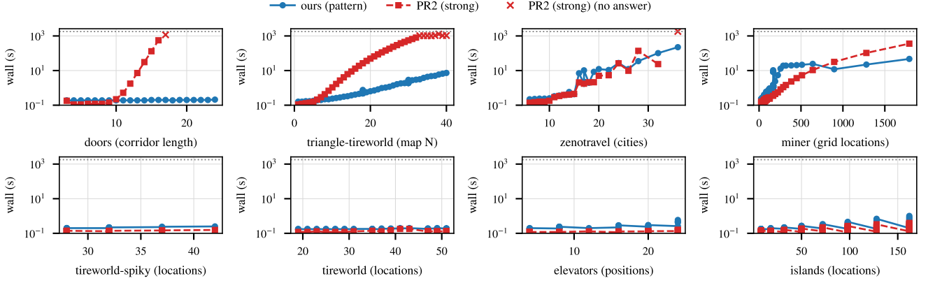
Figure 2: Scaling: wall time (s, log scale) against size, ours vs PR2; dotted line = 1,800 s cap. Filled = strong plan, cross = no strong-plan answer (timeouts/expiries).
