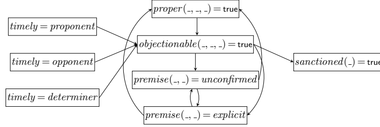
Fig. 2: Dependency graph fragment of the event description for ARG. Underscores denote variables grounded on input entities, action types or agent roles.
