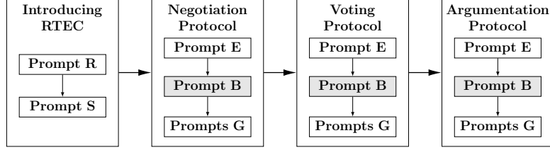
Fig. 3: genRTEC: LLM prompting for executable MAS specification generation. In this illustration, genRTEC is used for the construction of the specifications of a negotiation protocol, a voting protocol and an argumentation protocol. Prompt B is optional.
