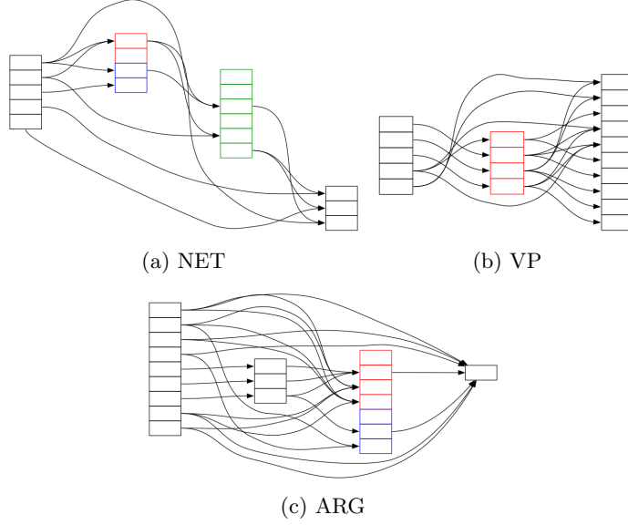
Fig. 4: The dependency graphs of the hand-crafted specifications of NET, VP and ARG. To avoid clutter, we omitted the FVPs from the nodes and the edges in a cycle. The nodes in a cycle are coloured red, blue or green. We grouped together the nodes of the same level, i.e. NET has four levels, VP has three levels, and ARG has four levels.
