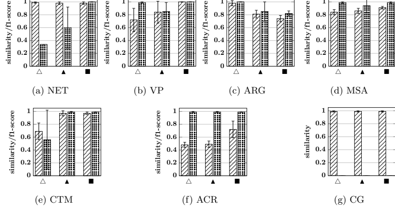
Fig. 5: Syntactic similarity (line-hatched bars) and f1-score (dotted bars) of genRTEC-constructed specifications compared to ground truth specifications. ‘ \triangle ’, ‘ \triangle ’ and ‘ \blacksquare ’ refer to the use of GPT, Gemini and Claude.
