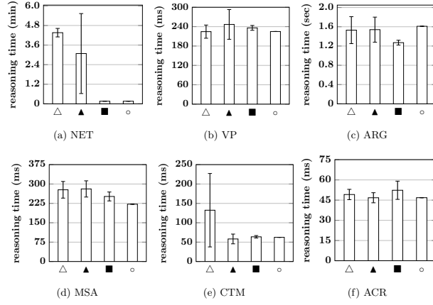
Fig. 6: Reasoning times of RTEC when operating on genRTEC-constructed specifications and ground truth specifications. ‘ \triangle ’, ‘ \triangle ’ and ‘ \blacksquare ’ refer to the use of GPT, Gemini and Claude, and ‘ \circ ’ refers to the ground truth specifications. The ranges of values in the vertical axes differ.
