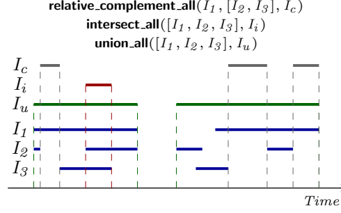
Fig. 1: Interval manipulation constructs of RTEC. I_1 , I_2 and I_3 (resp. I_c , I_i and I_u ) are input (output) lists of maximal intervals.
