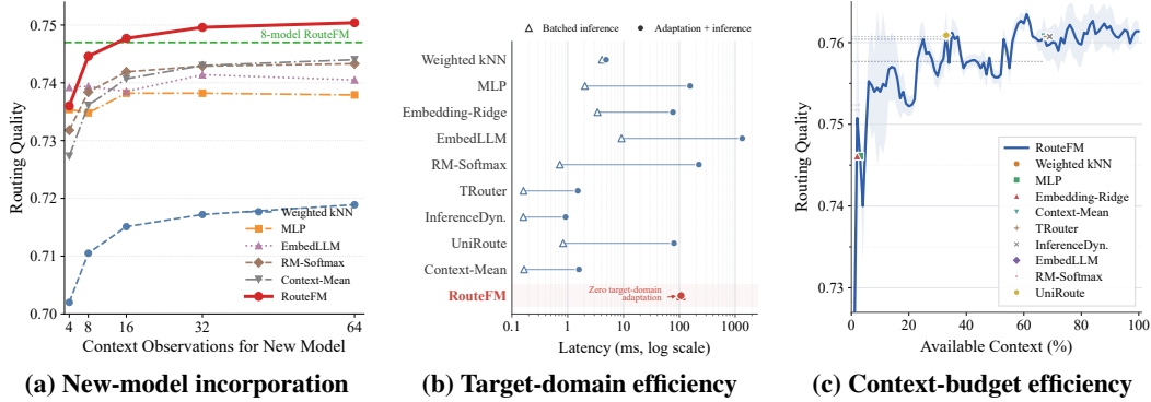
Figure 3: Adaptation of frozen RouteFM to deployment changes: (a) new-model incorporation, (b) target-domain efficiency, and (c) context-budget efficiency. Markers in (c) denote the context fraction required to match each baseline’s full-context routing quality.
