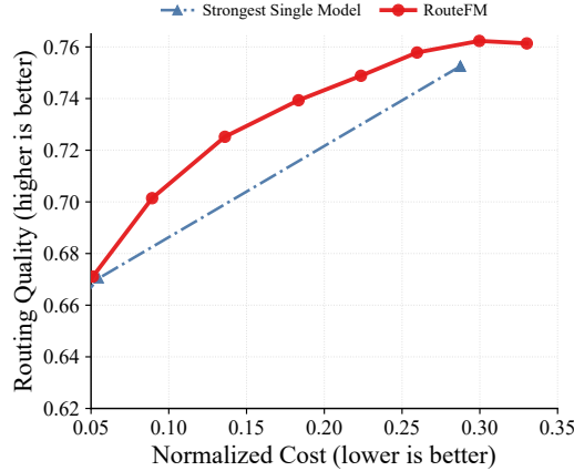
Figure A1: Quality–cost trade-off of RouteFM under different deployment preferences. Varying \lambda in the routing objective \hat{y}_m - \lambda \hat{c}_m produces different operating points without updating RouteFM’s parameters. The single-model baseline shows the corresponding quality–cost operating points obtained without routing.
