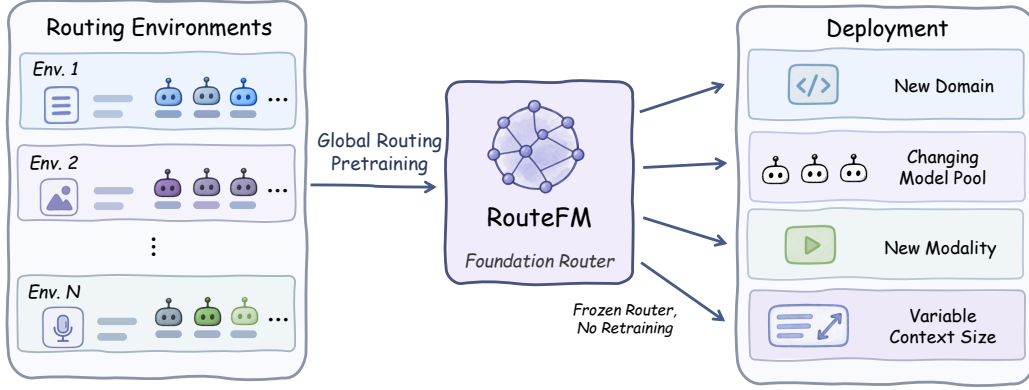
Figure 1: From local fitting to global routing pretraining. Traditional routers are optimized for individual routing environments, whereas RouteFM learns a reusable routing capability across heterogeneous environments and adapts to new environments through context.
