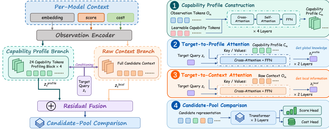
Figure 2: Architecture of RouteFM. Given behavioral observations for anonymous candidate models, RouteFM first constructs a compact capability profile for each candidate. The target query then retrieves complementary evidence from both the capability profile and the original behavioral context. These two representations are fused and jointly compared across the current candidate pool to predict target-specific quality and relative cost.
