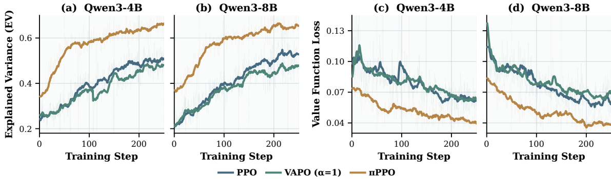
Figure 2: Critic explained variance (EV; a,b) and value-function loss (c,d) during training. Across Qwen3-4B and Qwen3-8B, \pi PPO consistently achieves higher EV and lower value-function loss than PPO and VAPO, with improvements evident from the early training steps.
