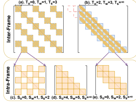
Figure 2: Visualization of the PSA parameterization that captures various attention sparse patterns.
