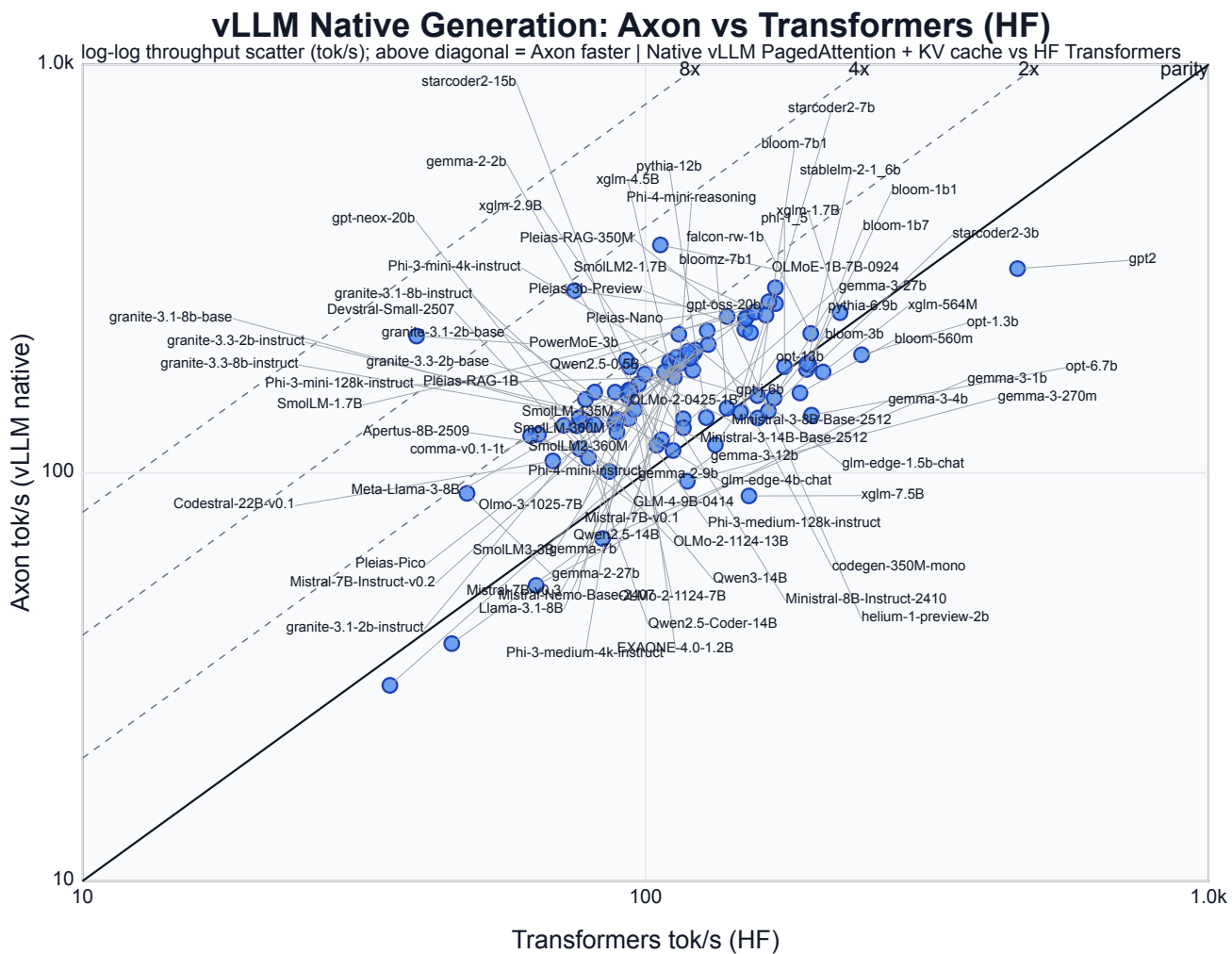
Figure 10: vLLM: Axon (vLLM native) vs. Transformers generation throughput on 88 checkpoints. Points above the parity line indicate Axon is faster. 74% fall above.
