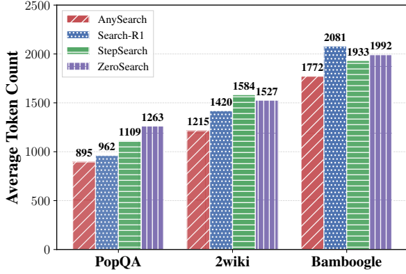
Figure 3: Average token count across different benchmarks on Llama-3.1-8B-Instruct. Here, the token count is the sum of output token and retrieved token.
