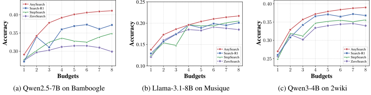
Figure 4: Performance of RL-based methods across varying budgets. We report the accuracy curves for (a) Qwen2.5-7B-Instruct on Bamboogle, (b) Llama-3.1-8B-Instruct on Musique, and (c) Qwen3-4B on 2wiki. For tool-free baselines such as ZeroSearch, we define the budget as the max turn, set to B + 1 .
