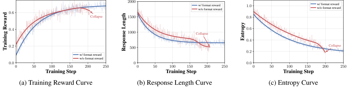
Figure 6: Training dynamics on Qwen3-4B showing the role of format rewards in training stability. (a) Without R_{format} , training reward rises initially but reverses around training step 175, while the full setting remains stable. (b) The no-format variant undergoes a sharp response-length reduction around the same point, indicating degeneration into trivial short outputs. (c) Its policy entropy also collapses abruptly, whereas the full setting decays smoothly and retains exploration.
