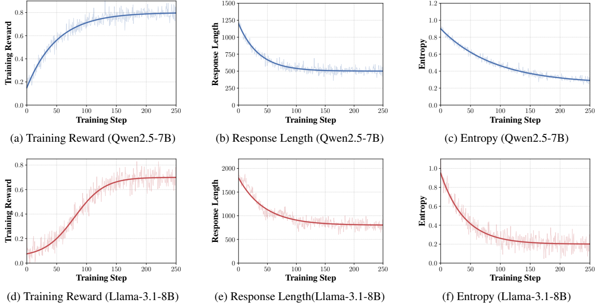
Figure 8: Training dynamics on Qwen2.5-7B-Instruct (top) and Llama-3.1-8B-Instruct (bottom), showing training reward, response length, and policy entropy across training steps.
