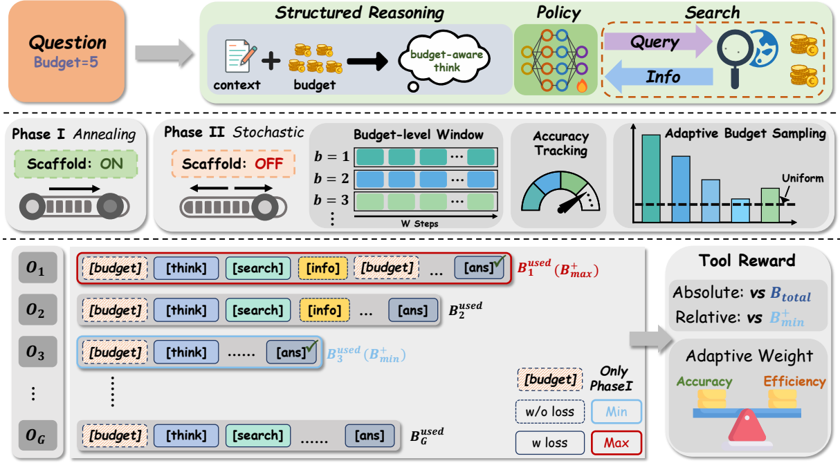
Figure 2: Overview of our framework. Phase I trains the agent with a reasoning scaffold and linearly decaying budgets to establish budget-aware decision patterns. Phase II removes the scaffold and applies sliding-window-based adaptive budget sampling and a composite reward with adaptive efficiency weighting.
