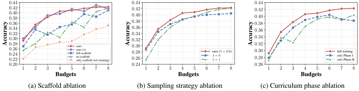
Figure 5: Ablation studies on HotpotQA with Qwen2.5-7B-Instruct across varying budgets. (a) Scaffold ablation. Full Scaffold uses scaffold in both Phase I and Phase II but removes it at inference; No Scaffold never uses scaffold in training or inference; Ours uses scaffold in Phase I, removes it in Phase II and inference; Ours (+Scaffold) applies our full training and retains the scaffold at inference; Only Scaffold uses scaffold at inference without any RL training. (b) Budget sampling strategy in Phase II, comparing \lambda=0 , \lambda=1 , and Ours ( \lambda=0.6 ). (c) Curriculum phase ablation, comparing training with only Phase I, only Phase II, and full training, all trained for 500 steps.
