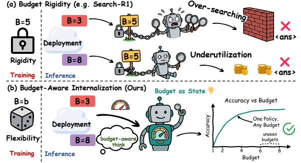
Figure 1: Comparison of search behaviors under varying budgets. Existing methods trained under fixed budgets cannot adapt their search strategy when the budget changes, while our method adjusts its allocation proportionally to the available budget.
