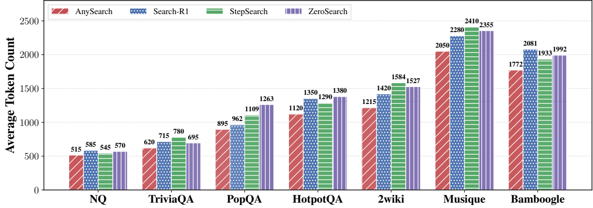
Figure 7: Average total token count across all benchmarks on Llama-3.1-8B-Instruct ( B = 5 ). Total tokens include output tokens and retrieved tokens.
