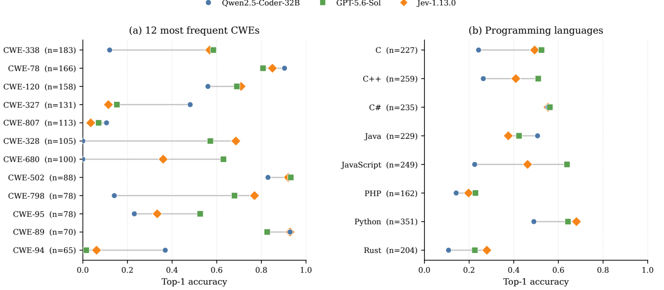
Figure 4. Top-1 classification accuracy of GPT-5.6-Sol, Jev, and Qwen2.5-Coder-32B-Instruct. Left: the 12 most frequent CWE classes in the benchmark, with class support shown in parentheses. Right: results grouped by programming language, with subset size shown in parentheses. The language-wise comparison is descriptive because programming-language subsets contain different mixtures of CWE classes.
