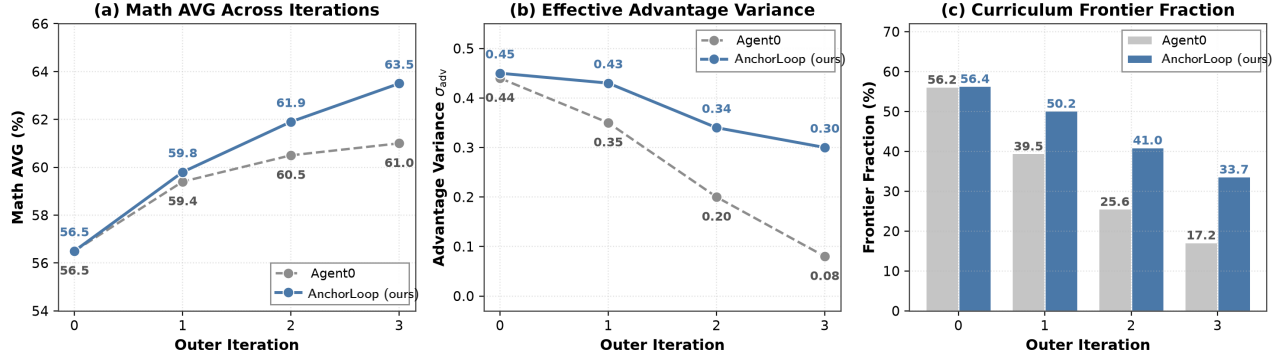
Figure 4: Iteration dynamics on MiMo-7B-Base. (a) Math AVG across the three outer iterations. (b) The within-group variance of effective advantages, V_{adv} , averaged over sampled groups in the Executor stage. (c) The reported Curriculum frontier fraction, defined as the fraction of generated tasks with a positive sampled agreement gap under Appendix B.3. An unresolved pair contributes zero.
