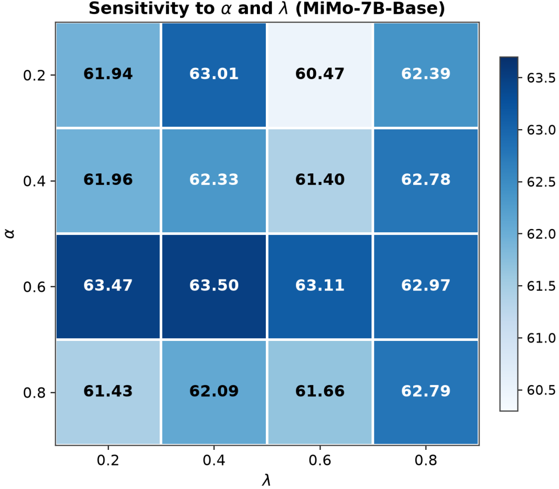
Figure 5: Hyperparameter sensitivity on MiMo-7B-Base, the appendix counterpart of Figure 3(b). Math AVG on a 4 \times 4 grid over the historical-advantage weight \alpha and the frontier reward weight \lambda . The peak at our default (\alpha, \lambda) = (0.6, 0.4) reaches 63.50, matching Table 1.
