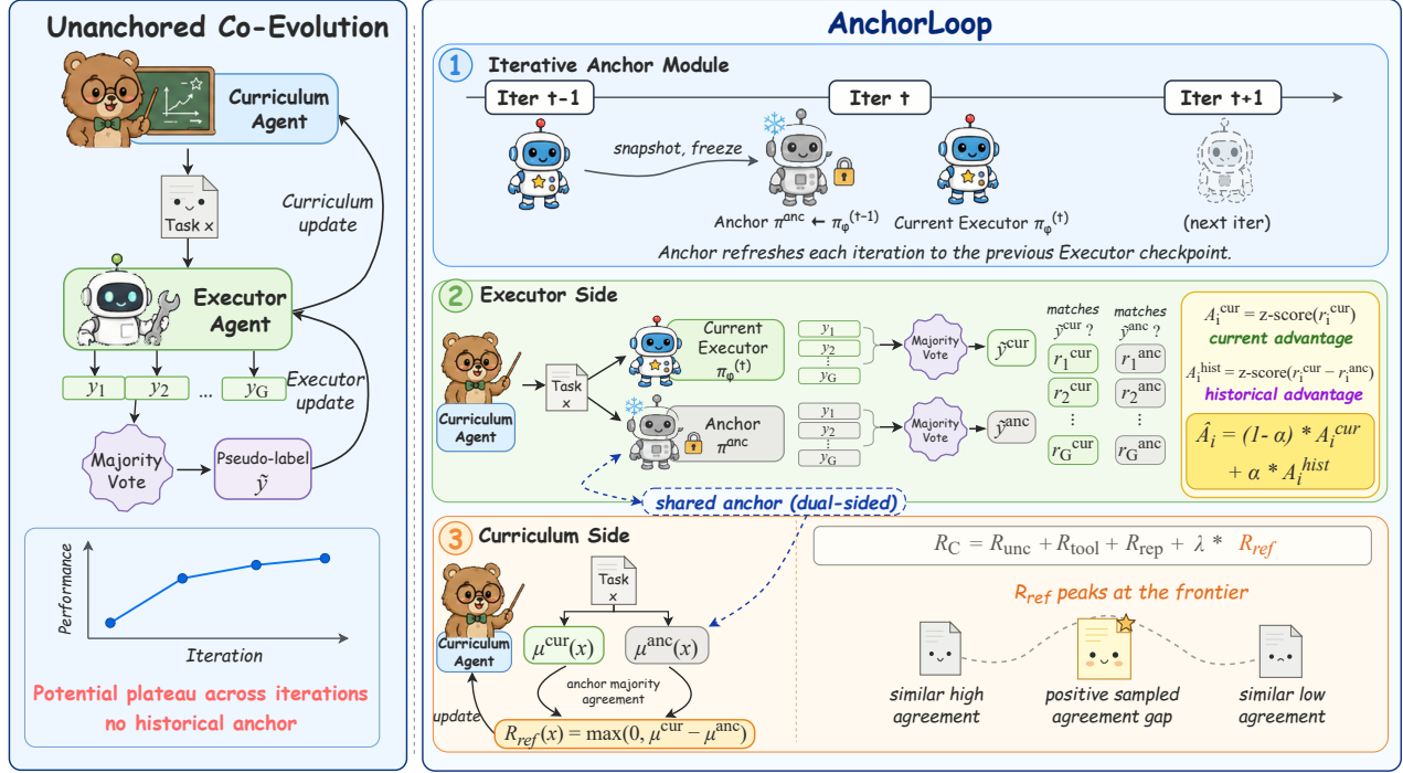
Figure 1: Overview of AnchorLoop. The left panel illustrates an unanchored two-agent self-evolution loop that can plateau. At outer iteration t , AnchorLoop copies the previous Executor into a frozen anchor and reuses it on both sides of the loop. During Curriculum training, the current Executor and anchor have identical parameters but produce independent rollout groups for the agreement-based reference reward. All format-valid tasks form the same-iteration task pool \mathcal{D}_t . During Executor training, the anchor remains fixed while the current Executor is updated. Current groups are resampled at every inner step, whereas one anchor group per task and Curriculum batch is cached and reused to construct the cross-reference advantage.
