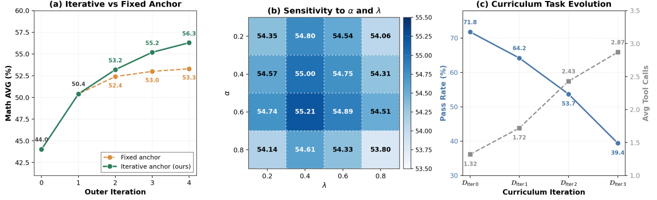
Figure 3: Anchor and Curriculum analyses on Qwen3-4B-Base. (a) Math AVG across outer iterations with an iterative anchor versus an anchor fixed to the base model. (b) Sensitivity over the historical-advantage weight \alpha and Curriculum reference weight \lambda on a 4 \times 4 grid; the default setting is (\alpha, \lambda) = (0.6, 0.4) . (c) Pass rate and average tool calls on 200 tasks sampled from each Curriculum stage. The iteration-1 Executor generates G = 8 trajectories per task, and both statistics are computed from the same 1,600 trajectories per stage.
