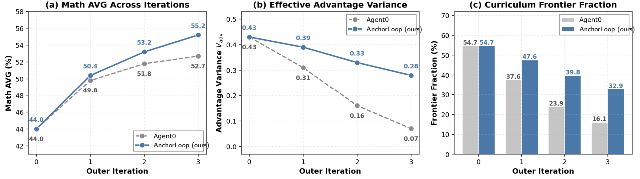
Figure 2: Training dynamics on Qwen3-4B-Base. (a) Math AVG across three outer iterations. (b) Within-group variance of the effective Executor advantage, V_{adv} , averaged over sampled groups. By iteration 3, it decreases to 0.07 for Agent0 but remains at 0.28 for AnchorLoop. (c) Fraction of Curriculum tasks with a positive sampled reference gap. An unresolved current–reference pair contributes zero. The fraction decreases from 54.7% initially to 16.1% for Agent0 and 32.9% for AnchorLoop by iteration 3.
