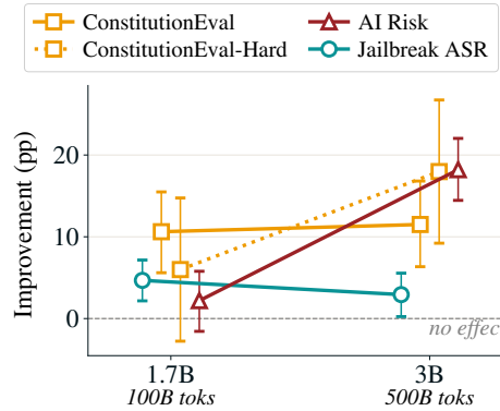
Figure 31: Improvement of SPP_{\{T0\}} over Vanilla across pretraining scales. Absolute improvement at the 1.7B/100B-token and 3B/500B-token scales. Gains on AI Risk and ConstitutionEval-Hard increase substantially with scale, while those on jailbreak ASR and ConstitutionEval remain roughly constant.
