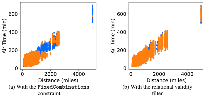
Figure 6. Operational correlation for real (blue) vs. augmented synthetic (orange) flight records: (a) distributional collapse resulting from the application of the FixedCombinations constraint; (b) uniform coverage achieved by replacing the constraint with the post-generation validity filter (Section D).
