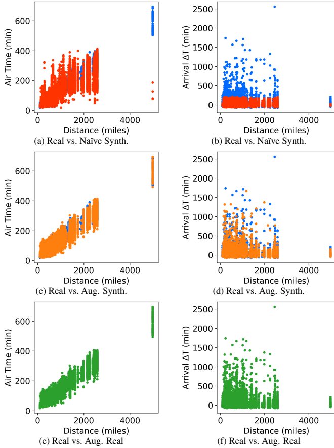
Figure 4. Operational correlation in real (blue), naïve synthetic (red), augmented synthetic (orange), and augmented real (green) flight records.
