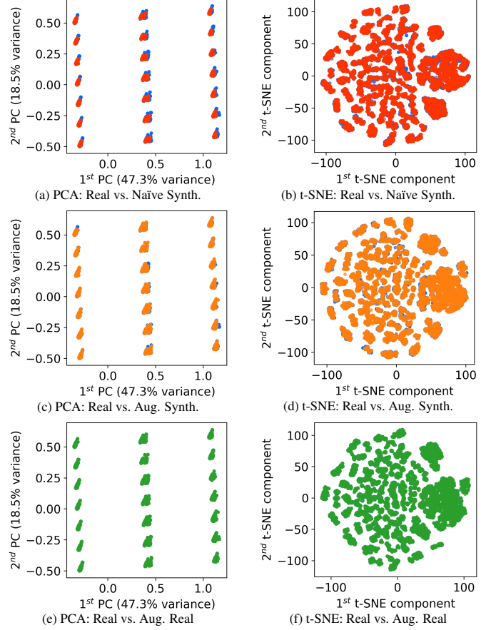
Figure 3. Diversity comparison of real (blue), naïve synthetic (red), augmented synthetic (orange), and augmented real (green) flight records.
