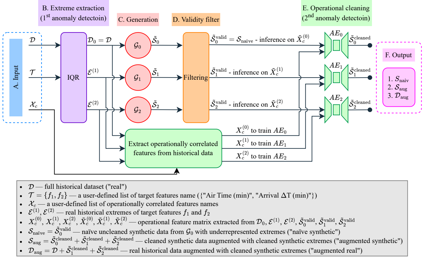
Figure 2. Overview of the TailBooster architecture with two target features.
