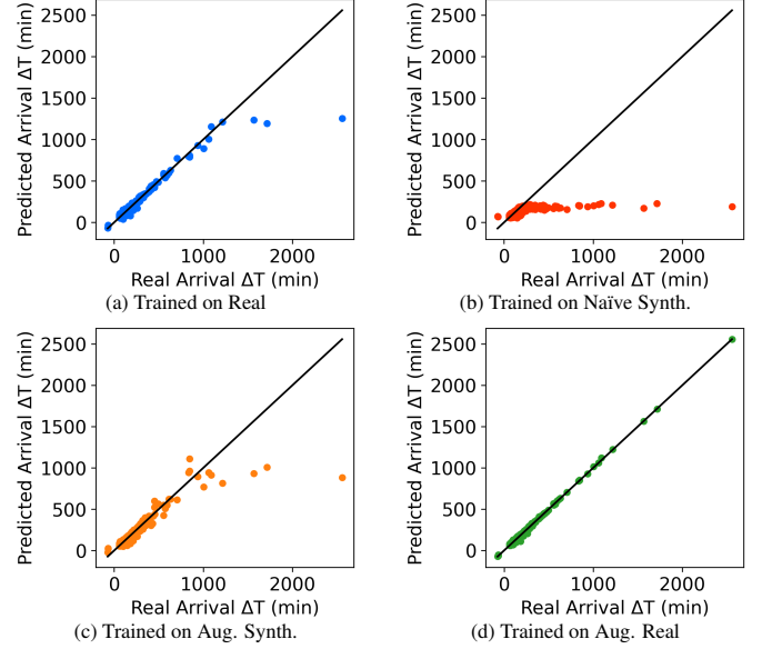
Figure 5. Predicted vs. real “Arrival \Delta T (min)” for XGBoost trained on the Real (blue), Naïve Synthetic (red), Augmented Synthetic (orange), and Augmented Real (green) datasets. The black diagonal represents perfect prediction.
