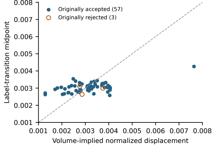
Fig. 1. Exact-distance boundary fits for the 57 objects accepted in the recorded analysis, replayed on the original queries. Left: object-specific fitted transitions (thin lines) and the transition at median fitted parameters (bold); zero marks the raw mesh. Right: label-transition midpoint versus volume-implied displacement, with identity line ( r = 0.58 ). Open markers show the three fits that failed the acceptance checks; they are excluded from the correlation.
