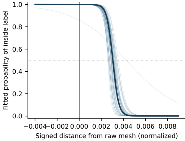
Fig. 1. Exact-distance boundary fits for the 57 objects accepted in the recorded analysis, replayed on the original queries. Left: object-specific fitted transitions (thin lines) and the transition at median fitted parameters (bold); zero marks the raw mesh. Right: label-transition midpoint versus volume-implied displacement, with identity line ( r = 0.58 ). Open markers show the three fits that failed the acceptance checks; they are excluded from the correlation.
