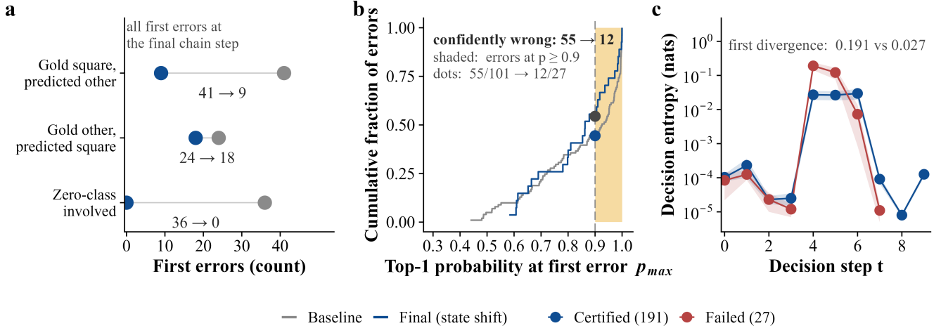
Fig. 4. Composition, confidence, and uncertainty of final-step errors. (a) All 101 baseline first errors sit at the chain’s final step, and the 27 remaining errors of the final configuration are all table-lookup confusions between the square class and the other class, with all zero-residual verdicts correct (31/31). (b) Distributions of top-1 probability at the first erroneous decision step: the two configurations’ shapes nearly coincide, and confidently wrong decisions fall from 55 to 12; the state shift changes the number of errors, not their confidence. (c) Decision entropy along the chain: early steps are near-deterministic (below 0.001 nats), real uncertainty concentrates in the last three steps, and failing problems have seven times the entropy of passing problems at the first divergent step (0.191 versus 0.027 nats).
