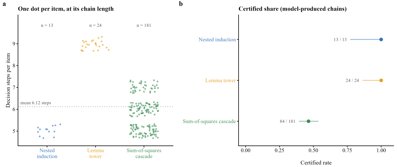
Panel (a): each item is one dot at its decision-step count (jitter within the bin); the cascade spreads 5-7 (71/72/38), the other two families are single-step. Panel (b): certified share of the model-produced chains with Wilson 95% intervals from k/n (0.77-1.00, 0.86-1.00 and 0.39-0.54); the gold-chain arm is 218/218 by construction.
