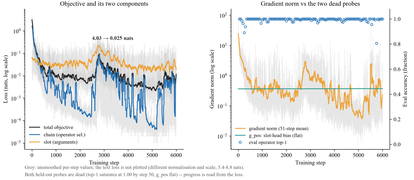
Fig. A1. Training dynamics of the final configuration (6,000 steps). (a) Total objective with the chain and slot components (log axis). (b) Clipped gradient norm and held-out operator top-1 accuracy; the latter saturates from step 50 onward, so training progress is read from the loss.
