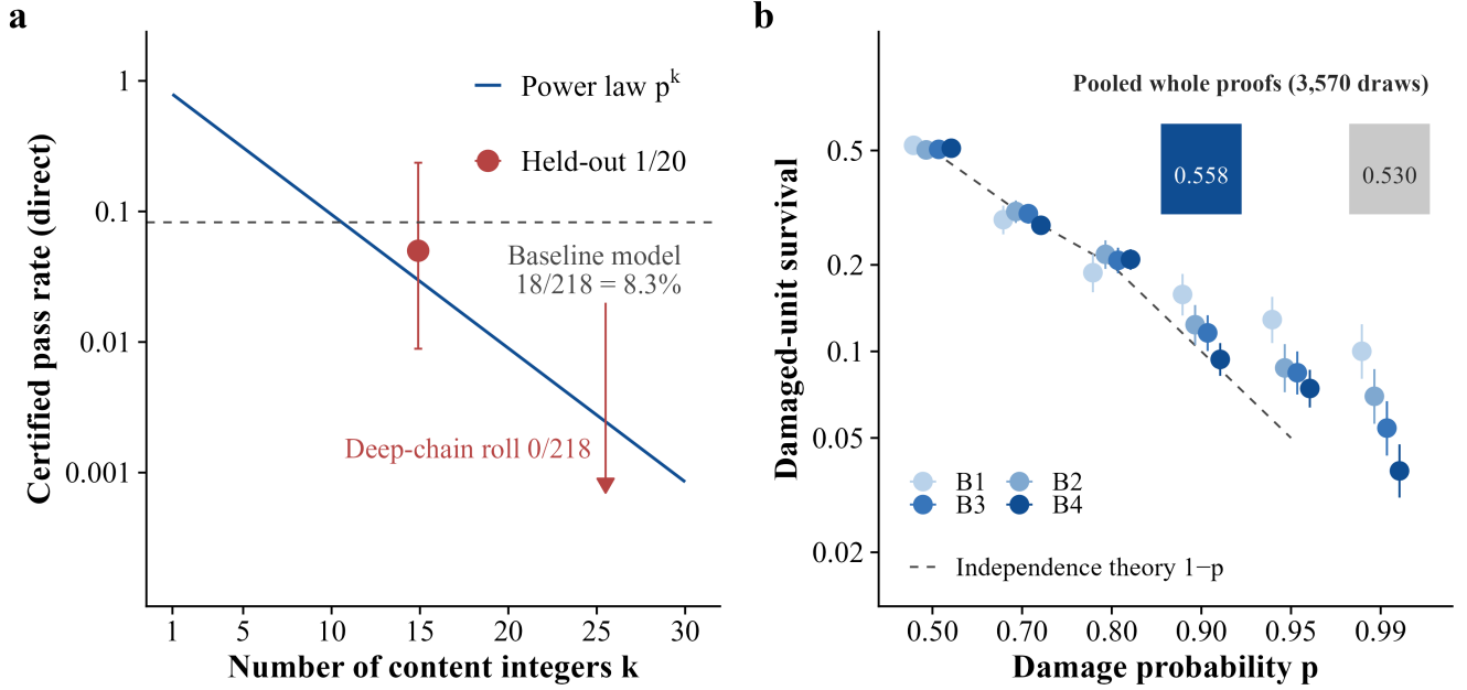
Fig. 3. Quantitative tests of Law 1. (a) The pass rate of direct generation decays as a power law in the number k of content integers ( p = 0.79 ), with measured points overlaid (control 1/20, deep-chain suite 0/218, comparison model 18/218). (b) Measured pass rate under controlled integer corruption (0.558) against the independent-assumption theory (0.530), bin by bin.
