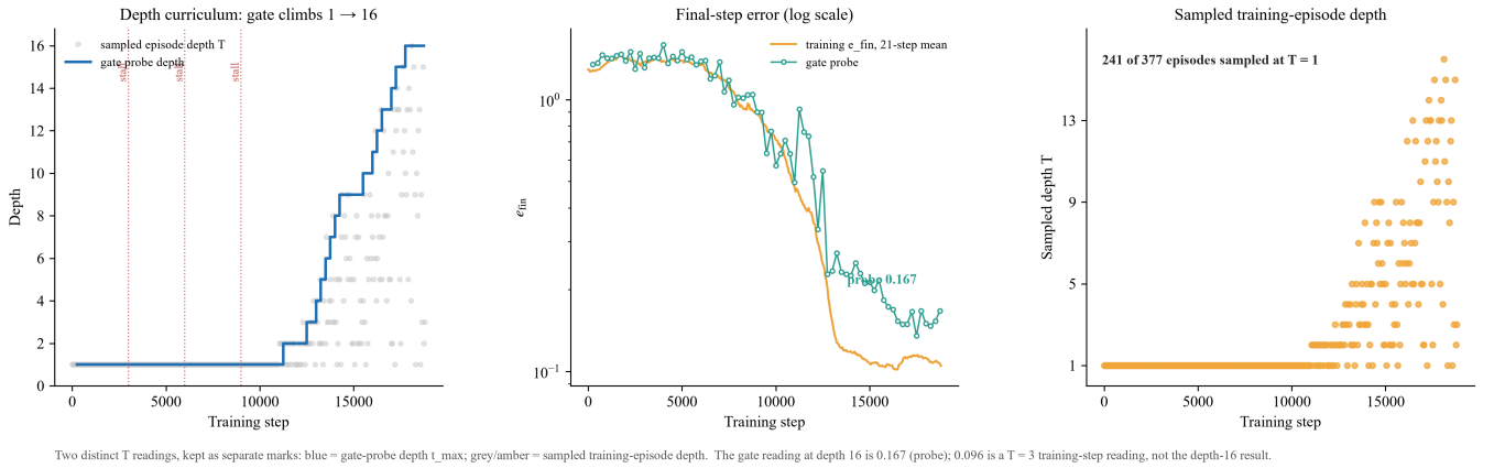
Fig. A2. The depth-curriculum ladder of the discretization experiment (v15). (a) The gate-probe measured depth rises monotonically from 1 to 16, with all fifteen openings between training steps 11,000 and 17,500; the shading shows depth sampling of training episodes. (b) Probe and training error curves. (c) Depth sampling of training episodes.
