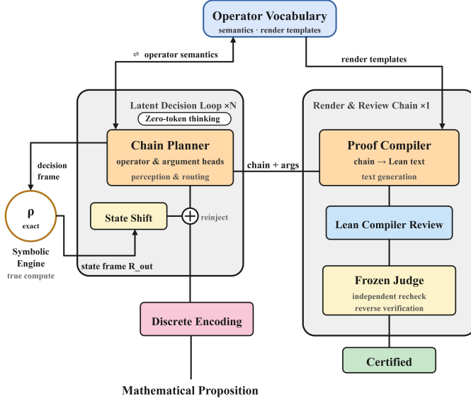
Fig. 1. The SCOPE architecture and data flow. A mathematical proposition enters a latent decision loop through discrete encoding: the chain planner, with its operator and argument heads, handles perception and routing and commits to one decision per step inside the operator vocabulary, which supplies both operator semantics and rendering templates; the symbolic engine executes each step exactly, and the state frame, after the state shift, feeds back into the decision loop, so multi-step thinking is carried endogenously by the loop with zero generated tokens (the Zero-token thinking label in the figure). The chain and its arguments go to the proof compiler, which renders Lean text from the templates; the Lean compiler reviews it, a frozen review program performs an independent recheck and reverse verification, and a certified proof is output.
