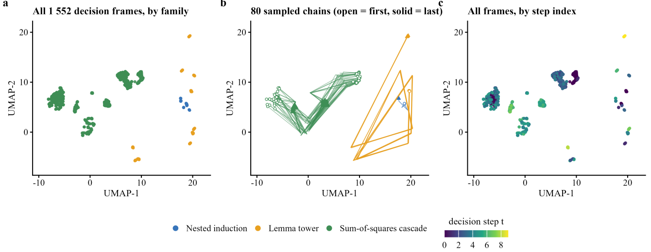
Frames are organised first by family -- the three families separate almost perfectly in the embedding (1-NN purity 0.999; chance level 0.659) -- and then by position in the chain: consecutive frames of one item share cosine 0.607 on average (5-95%: 0.431-0.790) against 0.154 for random frame pairs, all measured in the full 1152-d space.
