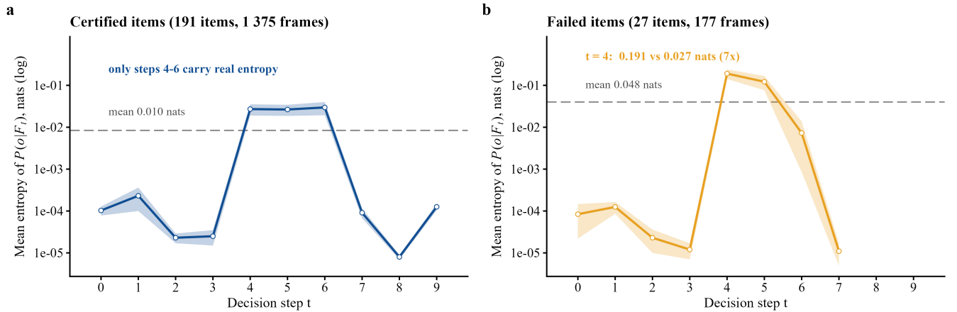
Entropy of the masked operator distribution P(o|F_t) -- the distribution the walk decides with. n per step: 191 certified frames (123 at t = 6 , 58 at t = 7 , 24 at t = 8-9 ); 27 failed frames (11 at t = 6 , 4 at t = 7 ). The model is measurably less certain where it goes wrong (0.191 vs 0.027 nats at t = 4 ), yet its top-1 probability there is still 0.918.
