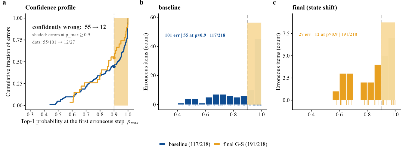
gen36 in-series pairing (baseline GEN35 vs final G-S), the same source and rule as Table 7; the s1 re-test reading (13/27) coexists and is not drawn. Panels (b) and (c): absolute counts per configuration (0.05-wide bins); the final configuration errs less often, not more humbly.
