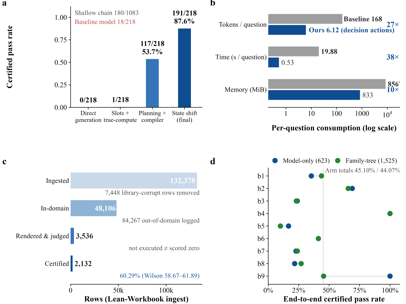
Fig. 5. Main results. (a) Certified pass-rate ladder of the main configurations: 0/218 (direct generation), 1/218 (slotting), 117/218 (compilation), 191/218 (state shift), with the shallow-chain reference 180/1083 and the comparison model 18/218 marked. (b) Resource comparison (log axis): generated tokens per problem (6.12 versus 168.0), wall-clock per problem (0.53 s versus 19.88 s), and peak memory (833 MiB versus 8,567 MiB); the comparison model runs one to two orders of magnitude higher on all three. (c) The three-tier triage funnel over the full Lean-Workbook library (132,378 → 48,106 → 3,536, with 2,132 certified). (d) End-to-end comparison of model-independent chain walking against type-tree chains over the nine extension families (45.10% versus 44.07%).
