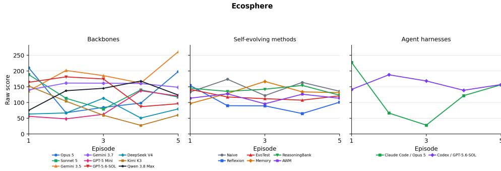
Figure 11: Ecosphere: raw-score learning curves within the scoring window.
