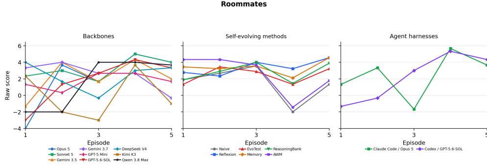
Figure 21: Roommates: raw-score learning curves within the scoring window.
