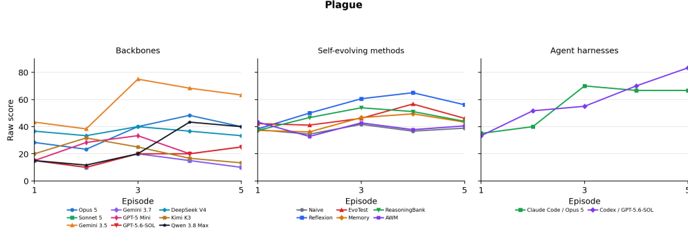
Figure 18: Plague: raw-score learning curves within the scoring window.
