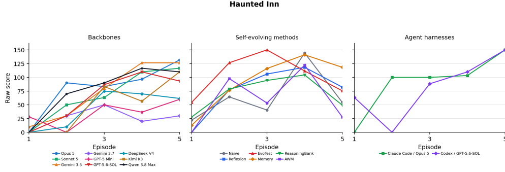
Figure 13: Haunted Inn: raw-score learning curves within the scoring window.
