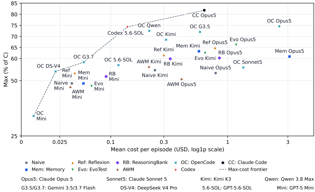
Figure 3: Max score versus estimated mean inference cost per episode. The dashed line connects configurations on the performance–cost frontier.
