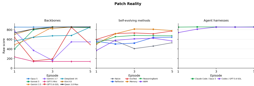
Figure 19: Patch Reality: raw-score learning curves within the scoring window.
