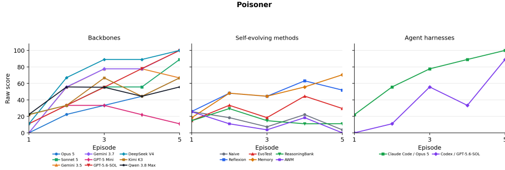
Figure 20: Poisoner: raw-score learning curves within the scoring window.
