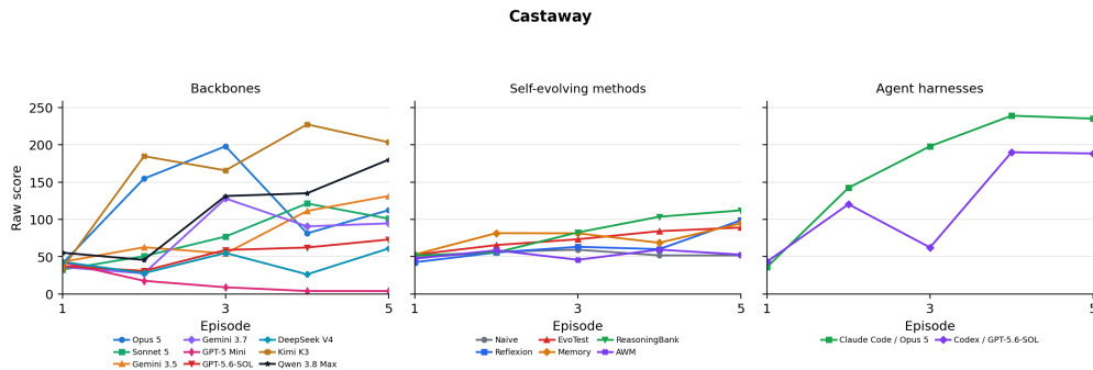
Figure 14: Castaway: raw-score learning curves within the scoring window.
