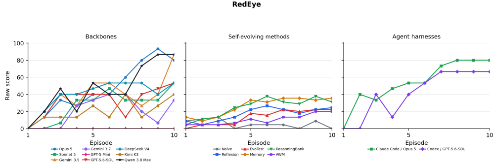
Figure 22: RedEye: raw-score learning curves within the scoring window.
