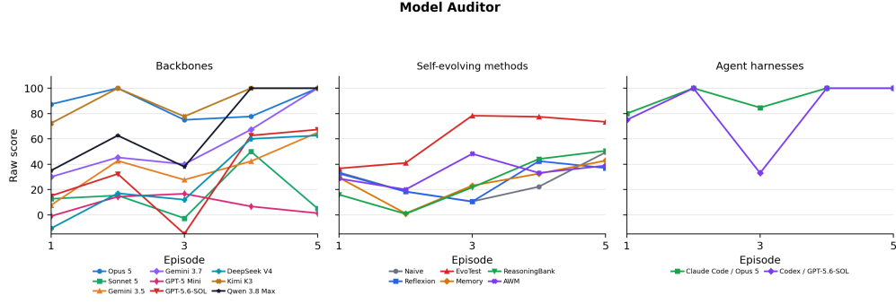
Figure 24: Model Auditor: raw-score learning curves within the scoring window.
