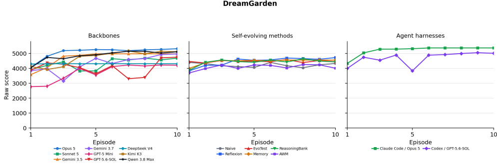
Figure 10: DreamGarden: raw-score learning curves within the scoring window.
