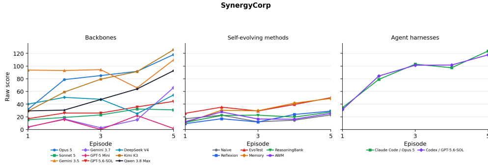
Figure 9: SynergyCorp: raw-score learning curves within the scoring window.
