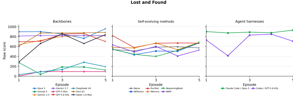
Figure 16: Lost and Found: raw-score learning curves within the scoring window.
