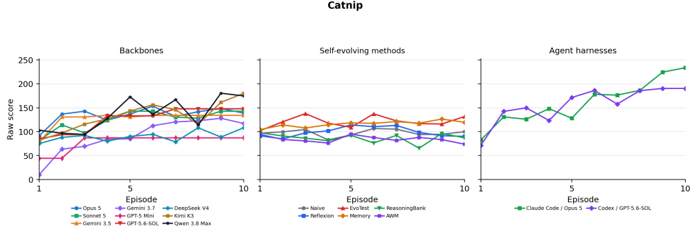
Figure 7: Catnip: raw-score learning curves within the scoring window.
