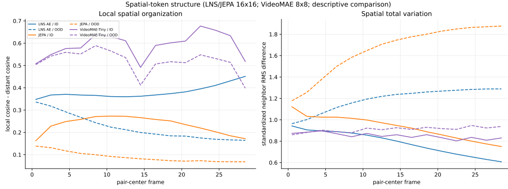
Figure 17: Native-token spatial organization on paired ID and far-OOD trajectories. Left: Local spatial organization. Local lift measures spatial locality; LNS exceeds JEPAs, while VideoMAE is highest descriptively. Right: Spatial total variation. Spatial variation grows most under JEPAs OOD, while ID becomes smoother.
