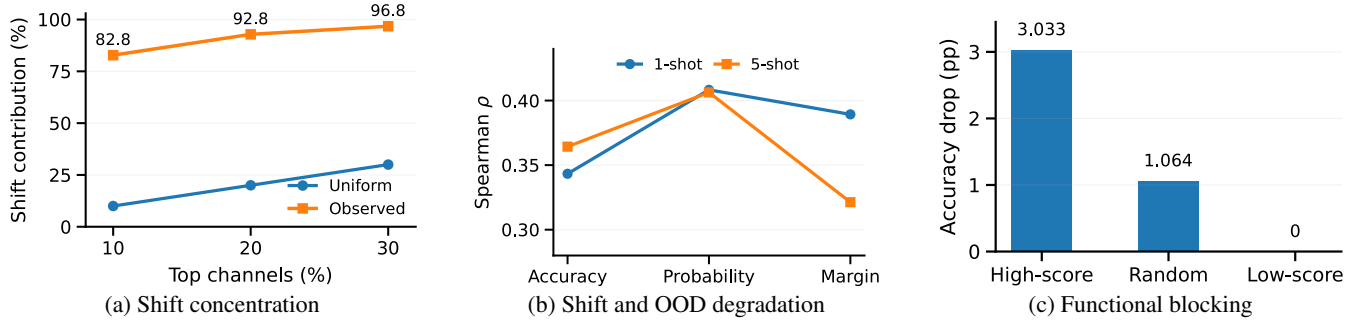
Fig. 4. Further analysis on ResNet12. (a) Cumulative contribution of channels with the largest null-corrected representation shifts. (b) Mean Spearman correlation across three seeds between episode-level shift mass and IID-to-OOD degradation for accuracy, confidence, and classification margin. (c) Accuracy drop after blocking the highest-scored, random, or lowest-scored 30% of channels while keeping the episodic classifier fixed.
