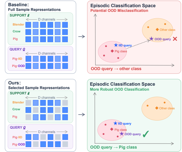
Fig. 1. Overview of few-shot classification under background shift. FULLREP passes all representation coordinates to a fresh episodic linear head; SAMPLESELECT independently masks each support and query example before fitting and prediction. The class-space plots are schematic, not measured embeddings.
