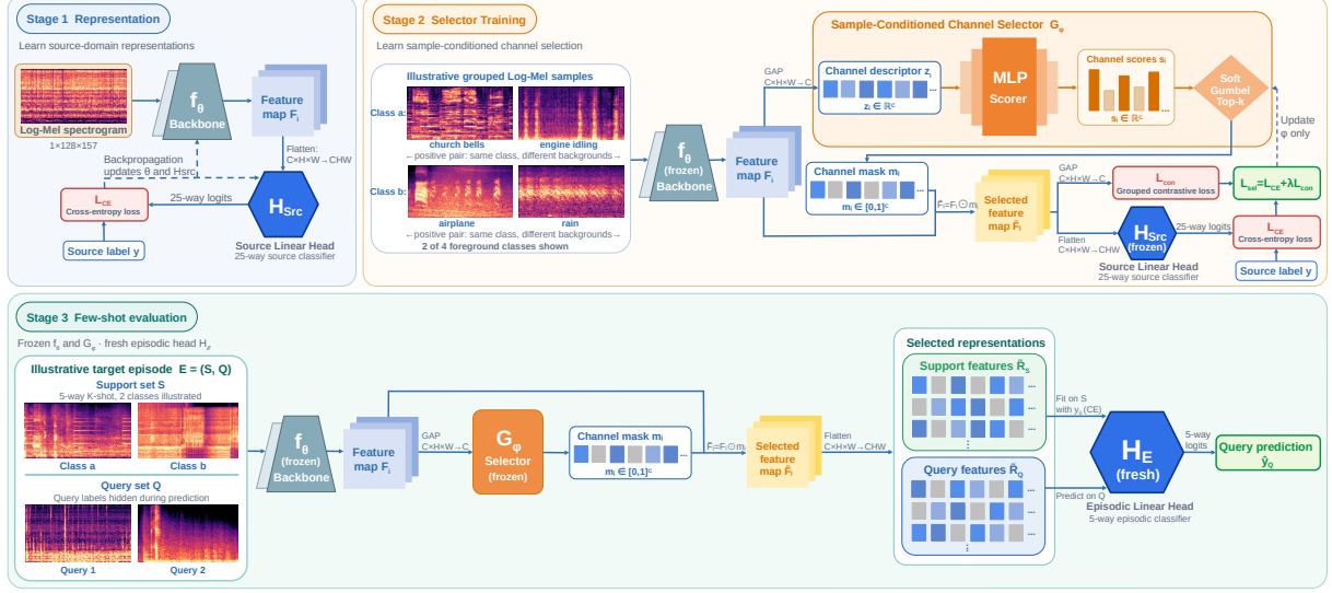
Fig. 2. Three-stage SAMPLESELECT pipeline. The source encoder/head are trained then frozen; the selector learns sample-wise masks with classification and cross-background contrastive losses; inference uses deterministic Top- k masks and a fresh support-only episodic head.
