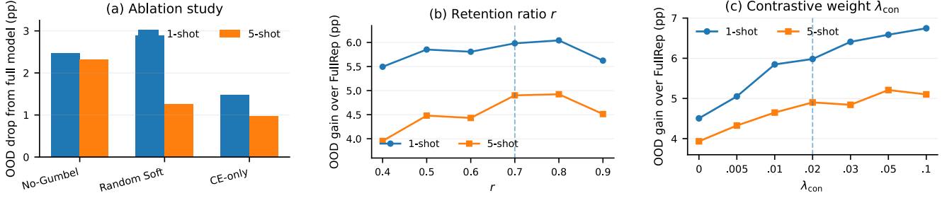
Fig. 3. Ablation and sensitivity analysis on ResNet12. (a) OOD accuracy drop after removing individual components of SAMPLESELECT. (b) OOD gain over FULLREP for different retention ratios r . (c) OOD gain over FULLREP for different contrastive weights \lambda_{con} . Dashed lines indicate the default settings used in the main experiments.
