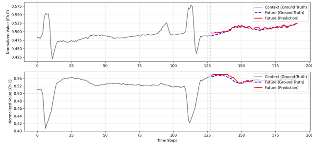
Figure 6: Zero-shot forecasting example on a randomly selected two-channel MIT-BIH sample under the 128/64 input/output setting. The gray curves denote the observed context, the blue dashed curves denote the ground-truth future, and the red curves denote SOTER’s predictions. The vertical dotted line marks the forecasting origin.
