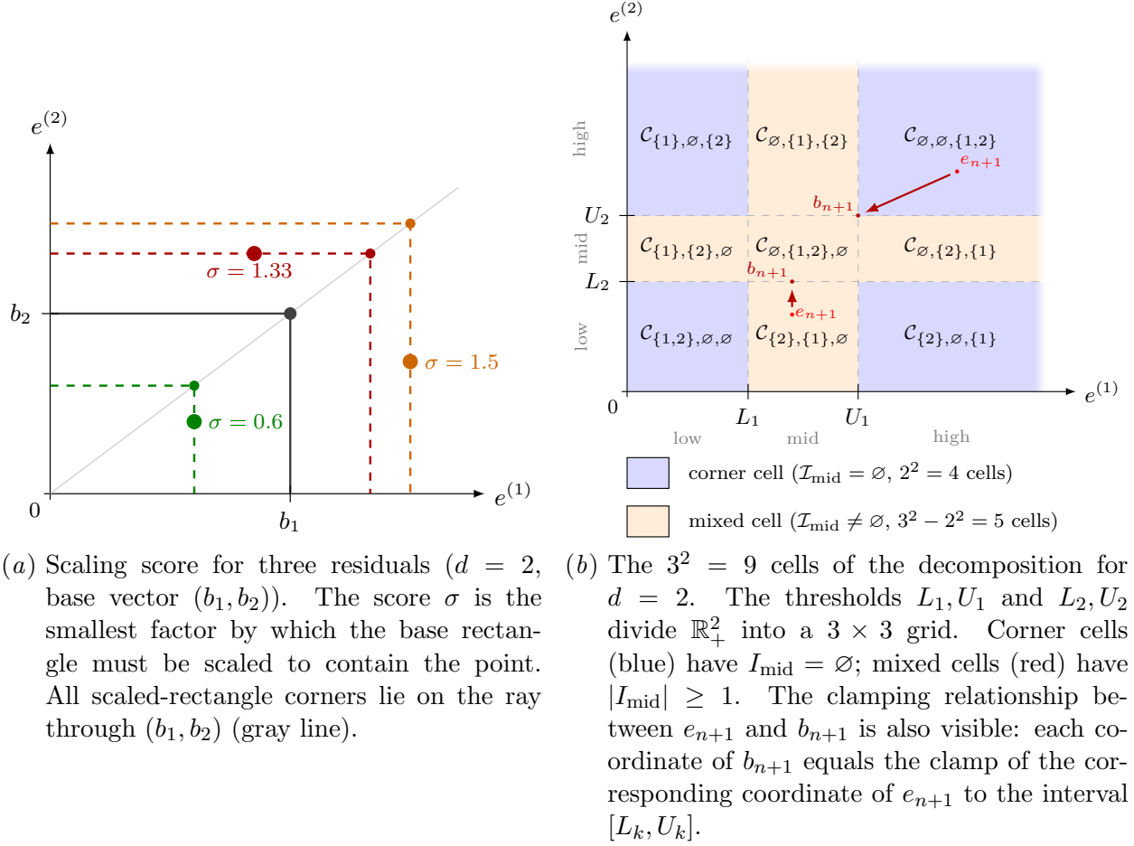
Figure 1: Scaling score and cell decomposition ( d = 2 ).
