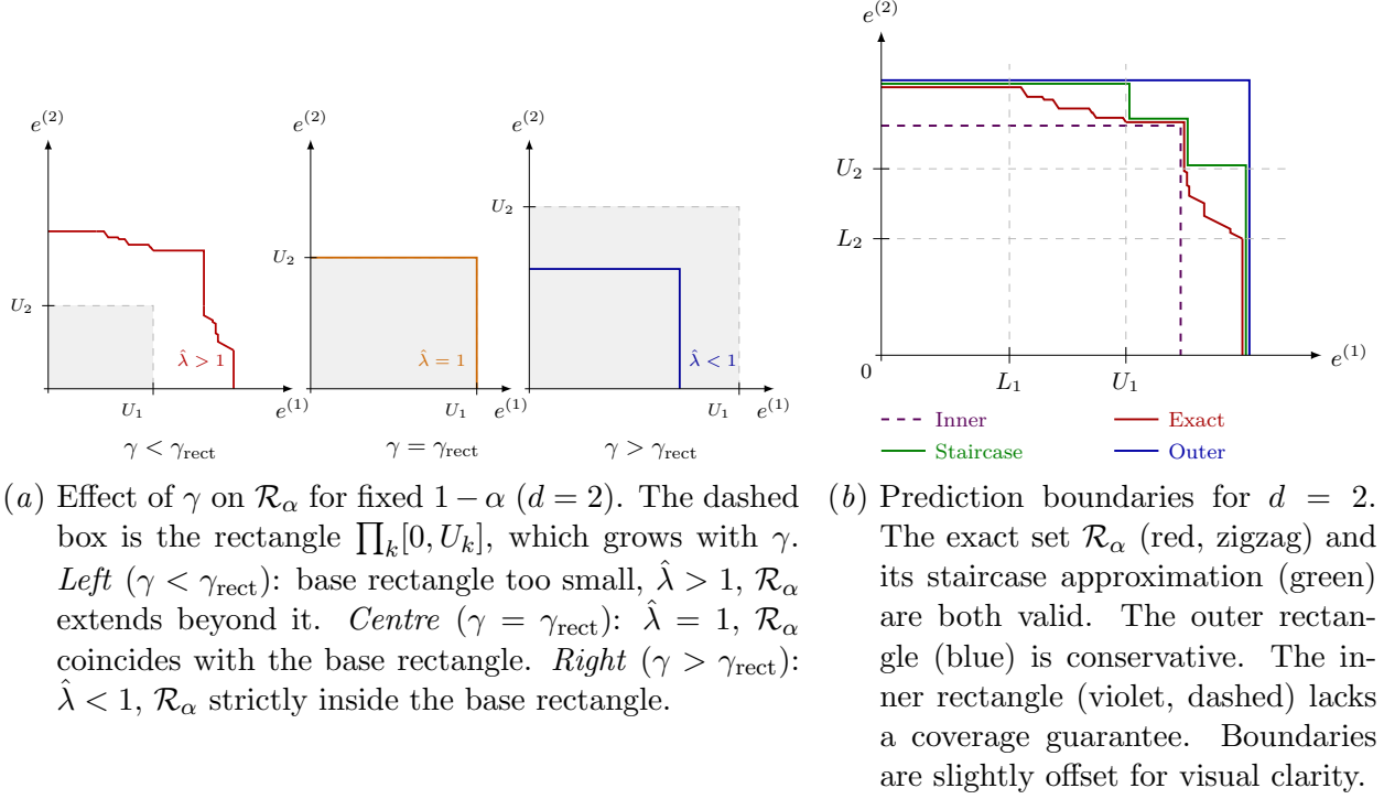
Figure 2: Effect of \gamma on the prediction region shape, and the four nested region types ( d = 2 ).
