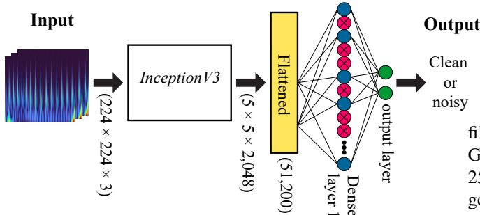
Fig. 3. Architecture of the final model. The three input images are identical. The red neurons in Dense layer 1 are prohibited by a dropout probability.
