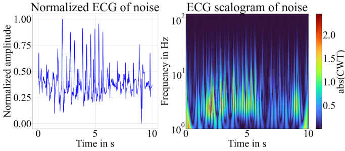
Fig. 2. Scalogram of a 10 s noise
