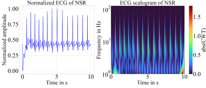
Fig. 1. Scalogram of a 10 s NSR
