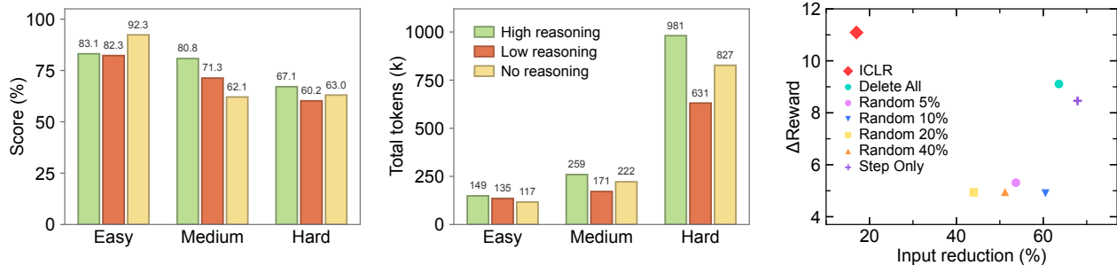
Figure 1: Reasoning utility and cost are state dependent. (a,b) Scores and token usage vary across reasoning settings and task difficulty. (c) Online interventions show a nonmonotonic reward-efficiency tradeoff. See Appendices J and F.
