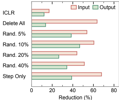
Figure 3: Trajectory amplification. Token savings do not track deletion.
