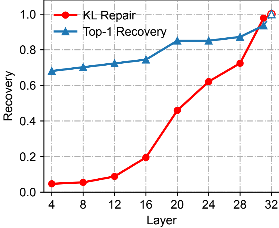
Figure 4: Activation patching across depth. Full history residuals progressively restore the perturbed next token distribution when they replace the corresponding deleted history residual at the prompt boundary.
