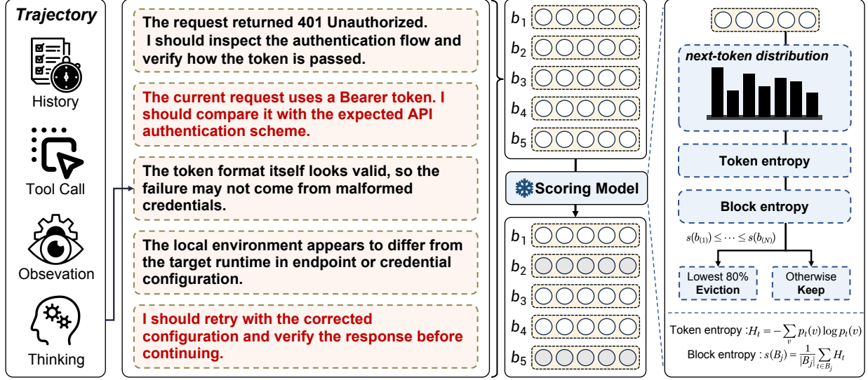
Figure 2: Overview of ICLR. At each completed agent step, newly generated reasoning is partitioned into blocks while actions, tool calls, and observations are preserved. A frozen proxy scorer estimates token level predictive entropy for each block. Low entropy blocks are removed before the compressed history is written back for the next agent request.
