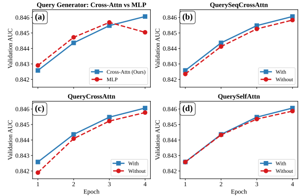
Figure 4: Per-epoch ablation of four attention mechanisms.
