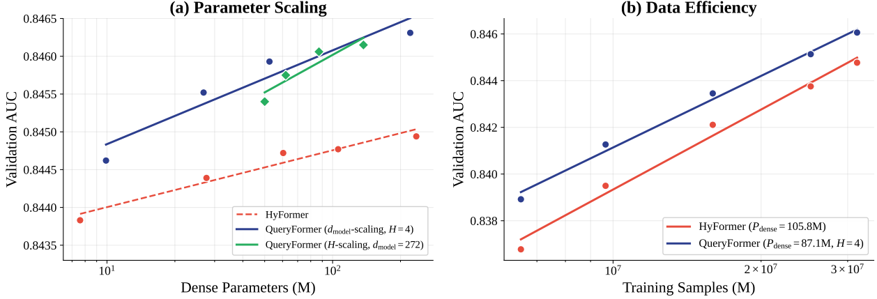
Figure 2: Scaling evidence for the stackable query-generation bridge. (a) Parameter scaling: QueryFormer traces a stronger AUC–dense-parameter frontier than HyFormer [8] within the explored budgets, with separate d_{\text{model}} - and H -scaling paths. (b) Data efficiency: QueryFormer ( P_{\text{dense}}=87.1\text{M} , H=4 ) remains above HyFormer ( P_{\text{dense}}=105.8\text{M} ) from about 20% to full training data. Both x-axes are logarithmic; P_{\text{dense}} denotes dense parameter count.
