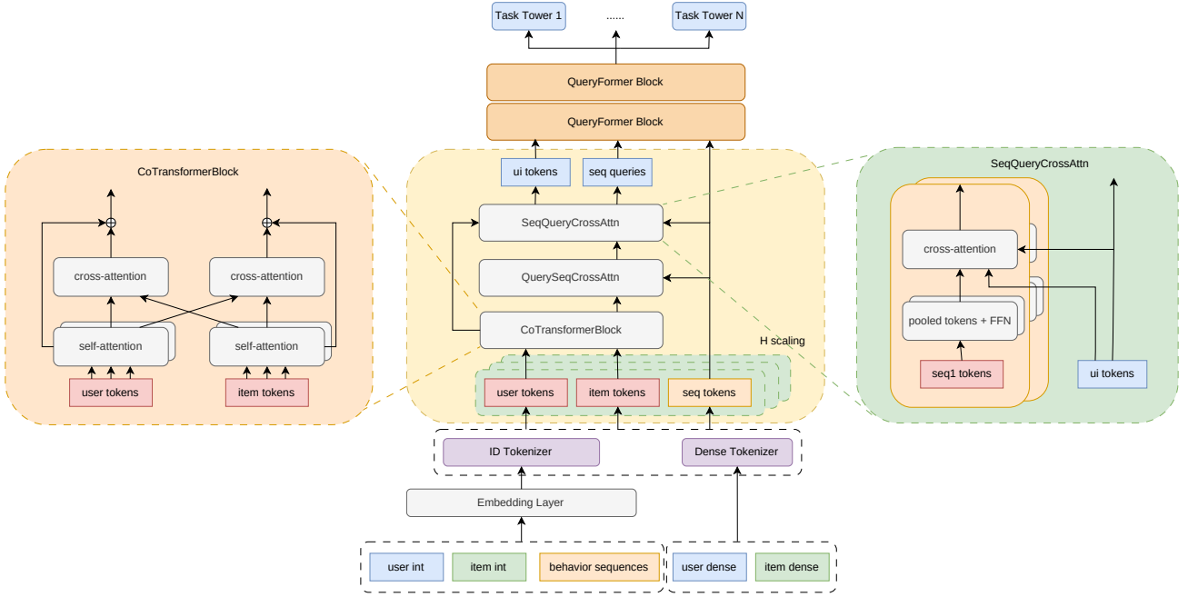
Figure 1: QueryFormer architecture. The reusable stackable query-generation bridge takes non-sequential field tokens and behavioral sequence tokens as input, returns generated query probes and mixed representations, and preserves the H dimension as parallel tokenization columns with shape- (B_s, H, T, d_{\text{model}}) views, where B_s is batch size and T is token count, before per-column outputs are combined.
