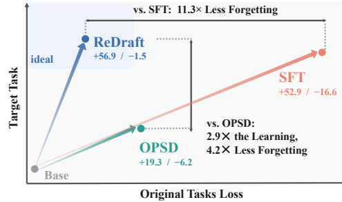
Figure 1: Target-task gain against loss on the original tasks, averaged over all experiments. ReDraft is in the upper-left region.
