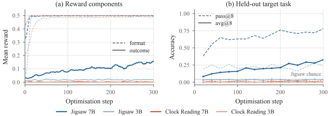
Figure 11: GRPO on the two cold-start tasks. (a) The two reward components during training. The format term reaches it in every setting, while the outcome term rises only for Jigsaw at 7B. (b) Accuracy on 100 held-out prompts, evaluated with 8 samples per prompt. The dotted line marks the accuracy of guessing a 2 \times 2 ordering at random.
