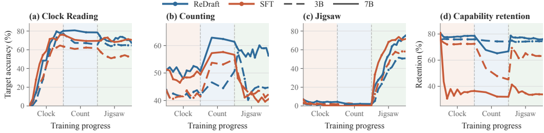
Figure 6: Sequential performance across all three target tasks. Panels (a–c) track Clock Reading, Counting, and Jigsaw throughout the complete curriculum; (d) shows original-task retention. Colour identifies the objective and line style the model scale. Backgrounds mark the active training stage.
