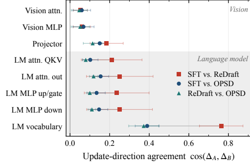
Figure 8: Agreement between the update directions of different methods, per module group. Markers are means over all pairs.
