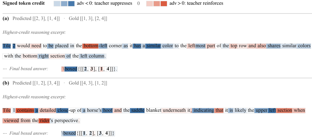
Figure 10: OPSD credit peaks away from the task-deciding answer. Token backgrounds show signed sampled-token credit: blue denotes \text{adv} < 0 (teacher suppression), red \text{adv} > 0 (teacher reinforcement), and darker colour larger |\text{adv}| under one shared scale.
