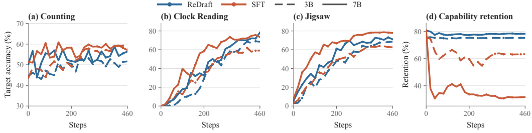
Figure 5: Mixed training at both model scales. All three target corpora are interleaved in a single run. Colour identifies the objective and line style the model scale. Panels (a–c) track the three target tasks separately; (d) shows original-task retention over 8 benchmarks.
