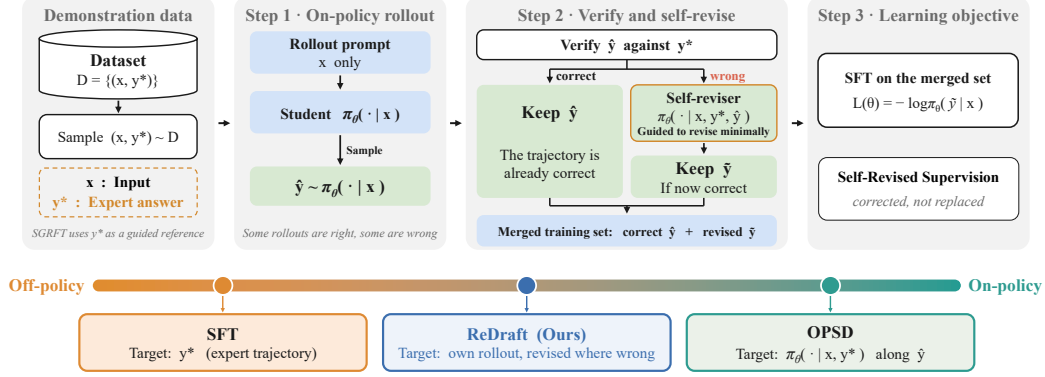
Figure 2: Overview of ReDraft. Each round samples a response from current policy, revises incorrect responses using an expert response as reference, verifies the revisions, and fine-tunes on the resulting targets. By explicitly incorporating the necessary corrections, ReDraft combines explicit target supervision with policy proximity .
