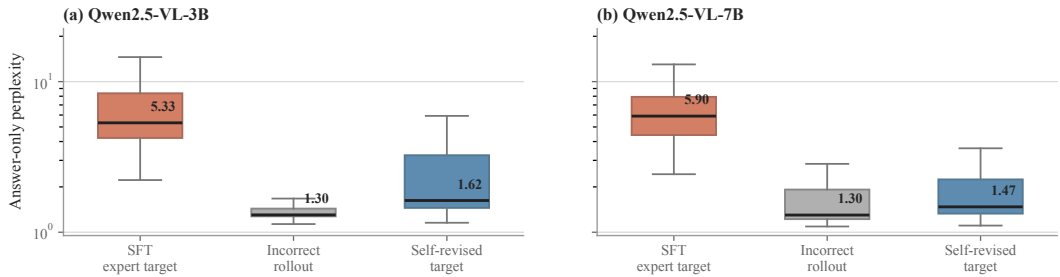
Figure 7: Self-revised targets are more policy-proximal than external SFT targets. Answer-only PPL is computed under the corresponding frozen base model and shown on a logarithmic scale; each box pools 400 paired examples from each of three tasks.
