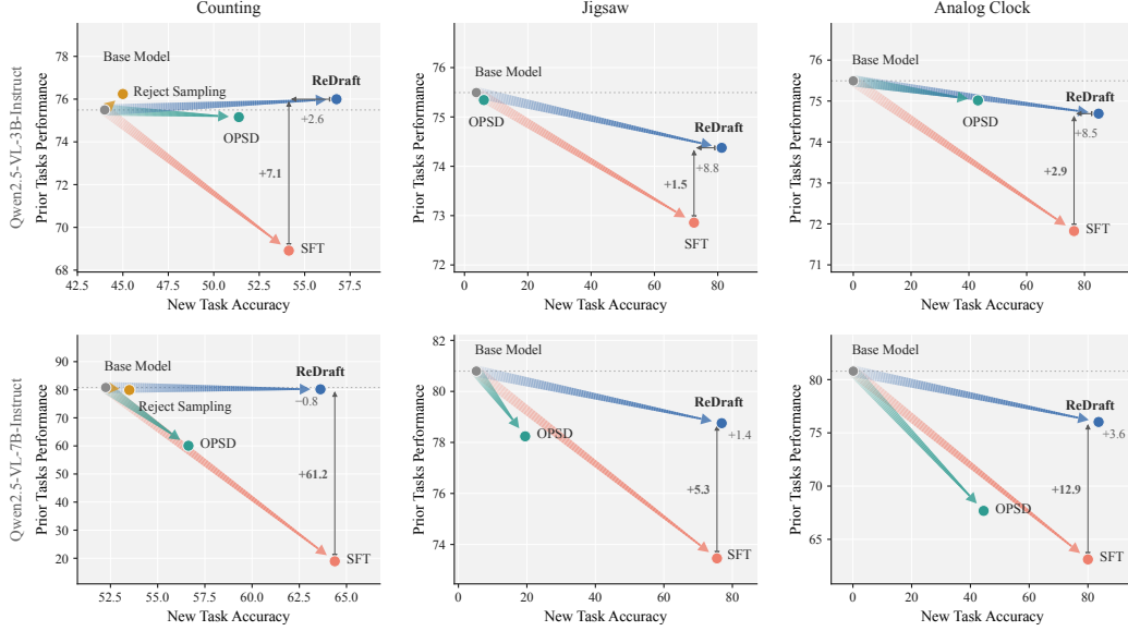
Figure 4: Target-task acquisition vs. retention of prior capabilities. Rows show Qwen2.5-VL-3B/7B; arrows originate at the base model. Reject Sampling is evaluated only on Counting, where the base policy already has substantial competence. Brackets show the ReDraft–SFT difference; higher is better on both axes.
