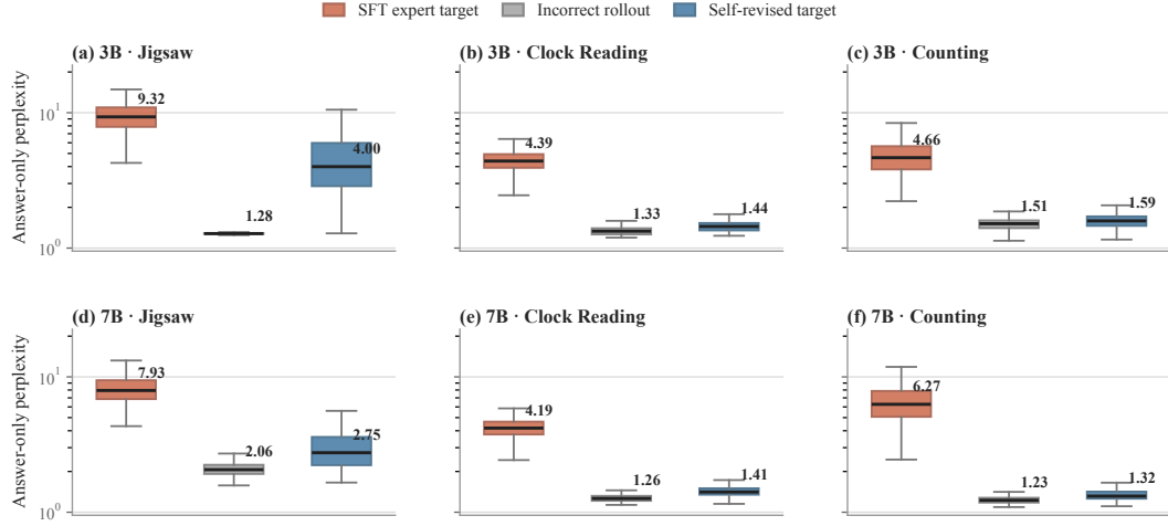
Figure 12: Per-task answer-only PPL distributions. Rows correspond to Qwen2.5-VL-3B/7B and columns to Jigsaw, Clock Reading, and Counting. Each panel contains 400 paired prompts per response source. Boxes span the interquartile range, centre lines and labels denote medians, and whiskers extend to 1.5 \times \text{IQR} .
