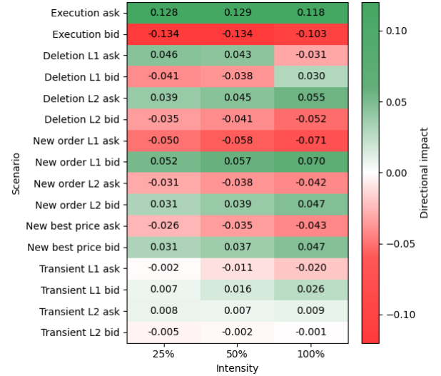
Figure 3: Average directional impact across scenario types and intensities. Positive values indicate a shift upward in mid-price and negative values indicate a downward shift.
