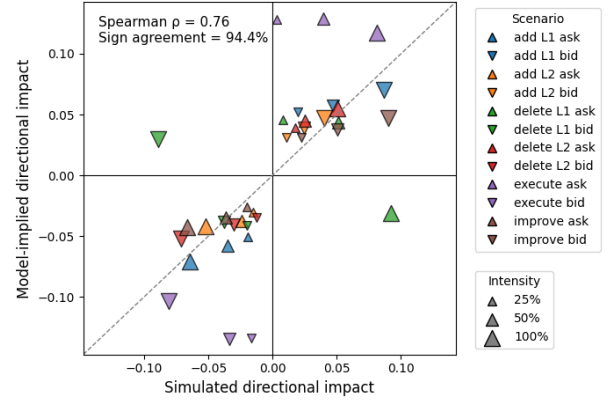
Figure 1: Model-implied versus simulator-defined average directional impact across parameterized scenarios.
