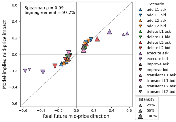
Figure 2: Distribution of model-implied and realized mid-price direction.
