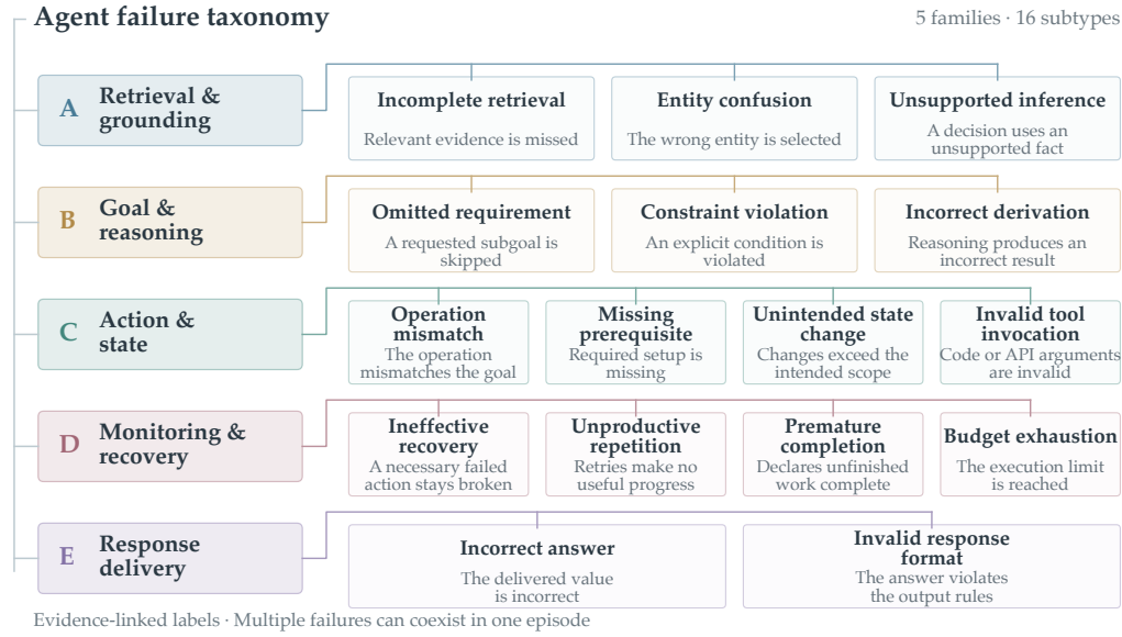
Figure 7: A hierarchy of observable agent failures. Five families organize evidence-linked deviations found in Qwen3.5-27B AppWorld trajectories. Each subtype identifies a distinct behavior or execution outcome. Labels can coexist within an episode. Recovery status is recorded separately.
