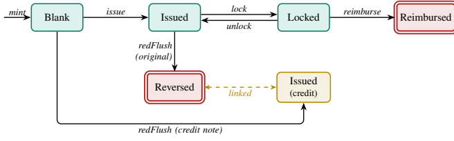
Fig. 1. Invoice lifecycle automaton \mathcal{L} (Def. 3). Double-bordered red states are terminal; the gold node is a frozen credit note. Tax declaration is an orthogonal one-way flag dc and is omitted for clarity.
