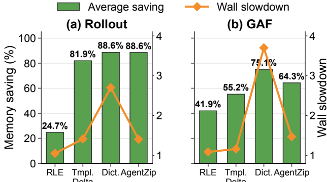
Figure 7. Effectiveness of AgentZip's codec portfolio.
