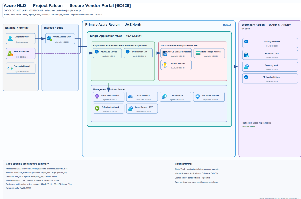
Figure 5: The generated architecture document in Project Falcon’s actual dossier. The diagram is review evidence, not an independently validated production design. Identity, application, data, monitoring, backup, and recovery elements contextualize the readiness example.
