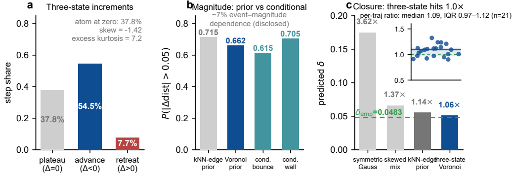
Figure A.12: The three-state structure of anchoring increments and the falsifiable closure of the \delta estimate (frozen measurements, AntMaze-medium rollouts). (a) Single-step increment shares: a 37.8% atom at zero (anchor unchanged), 54.5% advance, 7.7% retreat; the skew and excess kurtosis rule out any symmetric two-sided model structurally. (b) Retreat-magnitude read P(|\Delta_{\text{dist}}| > 0.05) under two priors and two conditionals; the Voronoi prior (0.662) sits within 7% of the bounce-conditional value (0.615), quantifying the event-magnitude dependence. (c) Four-model closure against the measured \delta_{\text{emp}} = 0.0483 (dashed): symmetric Gaussian 3.62\times , skewed mixture 1.37\times , kNN-edge prior 1.14\times , three-state Voronoi factorization 1.06\times ; inset: per-trajectory closure ratios (median 1.09, IQR 0.97–1.12, n=21 ).
