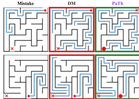
Figure 6: Qualitative comparison on mazes. When the path is directed into a dead-end, only PaTh is able to correctly revise it.
