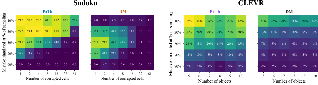
Figure 8: Recovery rate after corrupting a valid solution and re-noising it to a given point of the trajectory, on EXTREME MNIST Sudoku (left) and constrained scenes (right). The diffusion model recovers only within a narrow band, at the start of sampling on CLEVR and at 50% on Sudoku, and degrades sharply as mistakes accumulate. PaTh recovers throughout the region where change remains possible, declining only as less trajectory is left.
