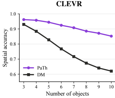
Figure 4: Spatial accuracy on CLEVR by scene size. The DM (238M) falls rapidly, while PaTh retains high accuracy.
