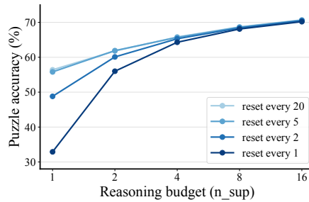
Figure 18: Puzzle accuracy against reasoning budget n_{\text{sup}} for different reset intervals. The Thinker’s state carries across denoising steps, improving accuracy by 23 points at low budgets.
