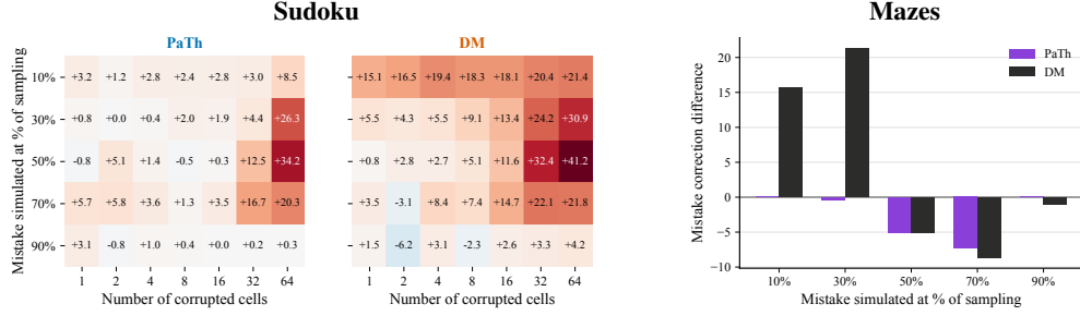
Figure 7: Difference in retention rate between indirectly and directly available mistakes on EXTREME MNIST Sudoku (left) and Mazes (right). The diffusion model retains the indirect mistakes far more often early in sampling, while PaTh treats the two types of errors comparably.
