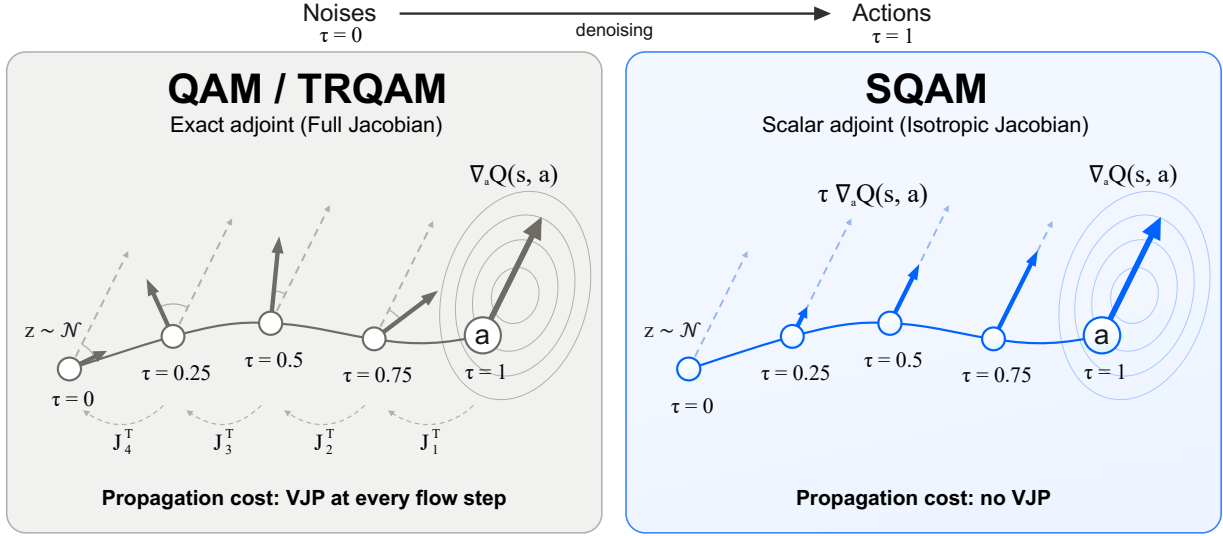
Figure 1: Adjoint matching propagates the critic’s gradient at the final action back to the flow steps that produced it, and the propagated gradient updates the flow model. Left: QAM and TRQAM integrate the lean adjoint ODE backward along the sampling chain, which takes a vector–Jacobian product J_i^T through the policy at every flow step, so the cost grows with the number of flow steps and the policy size. Right: SQAM instead scales the gradient at the final action, \nabla_a Q(s, a) , by the flow time \tau , with no vector–Jacobian product at any flow step.
