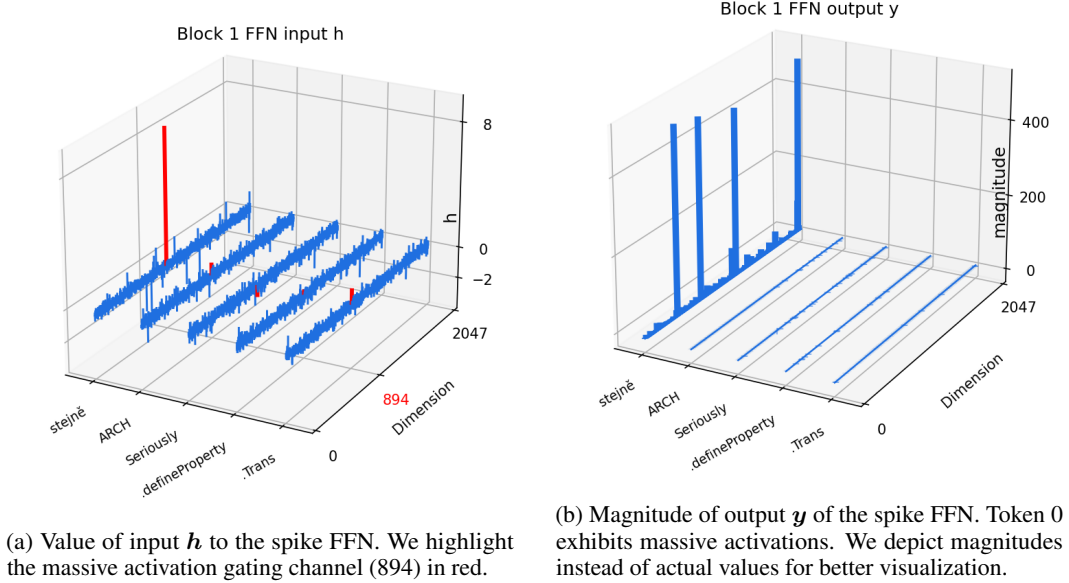
Figure 1: Inputs and Outputs of the Spike FFN.
