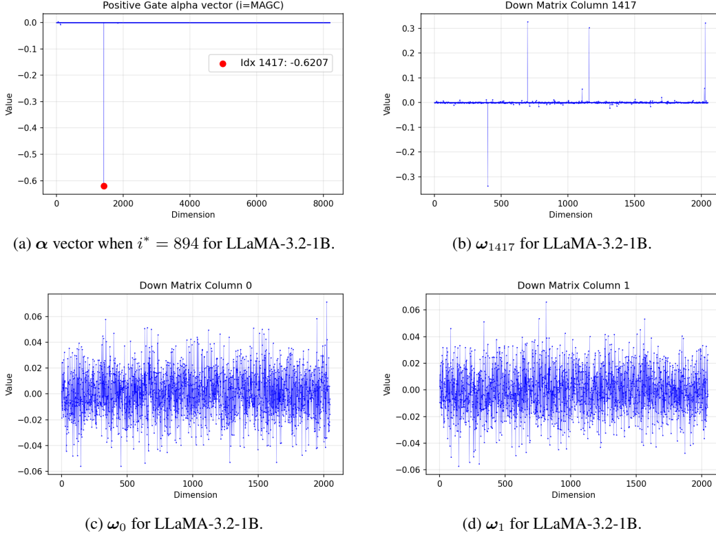
Figure 3: Visualization results for LLaMA-3.2-1B.
