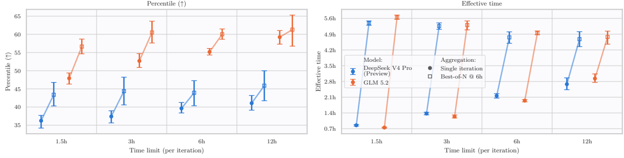
Figure 7 Impact of per-iteration time limits. Average percentile and effective-time obtained by Oneshot iterations under different per-iteration time budgets in the default29 set. Circled points represent single-iteration performance, while boxes indicate Best-of-N performance at six hour budgets. Error bars represent 95% CIs across our fixed 29-task set. The effective time measures the time taken for the run to finish. Best-of-N aggregates may remain below the target of 6h in the case of failing iterations that would exceed the maximum budget allocated.
