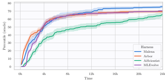
Figure 10 Left: oracle best-so-far vs. wall-clock time at Kimi K3 for Malena, Arbor, AiScientist, and MLEvolve. Right: per-run distribution of cumulative input, output(+reasoning), and modeled cache-read tokens, plus a USD-cost group at Kimi K3 pricing, for Malena, Arbor, AiScientist, and MLEvolve. MLEvolve’s cache group is omitted (always exactly 0, same reason as the GLM 5.2 figure).
