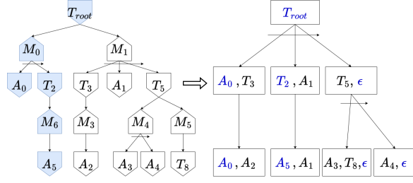
Figure 1: On the left, a simple decomposition schema in the form of an AND/OR tree, where T_i denotes abstract task i , M_i denotes method i and A_i denotes action i . On the right, we represent the corresponding cPDT. An identical potential solution for both structures is highlighted in blue.
