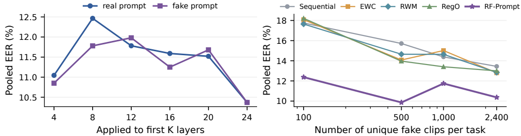
Figure 5: Protection-depth sweeps (left) and limited-fake-data adaptation (right). The other constraint remains active across 24 layers; the right axis counts unique fake clips per task.
