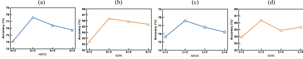
Figure 7: The effect of varying hyperparameters. (a) and (c) are experiments on ABIDE dataset. (b) and (d) are experiments on ADNI dataset.
