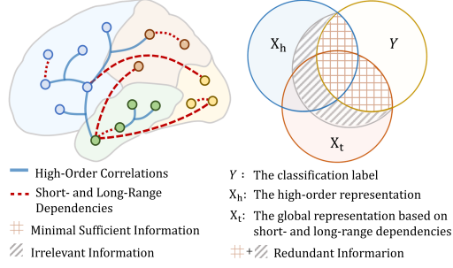
Figure 1: The brain network contains extensive high-order correlations as well as short-range and long-range dependencies. Multi-source information fusion, guided by the information bottleneck, aims to optimize the fused representation by capturing the minimal sufficient information from high-order representation X_h and global representation X_t for predicting the classification label Y .
