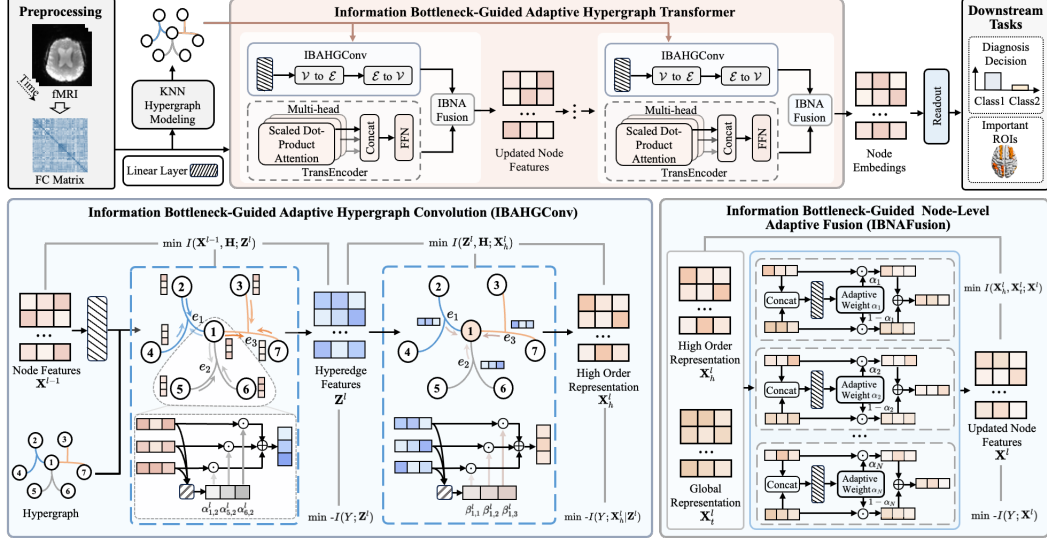
Figure 2: The overall framework of the proposed IBAHGT.
