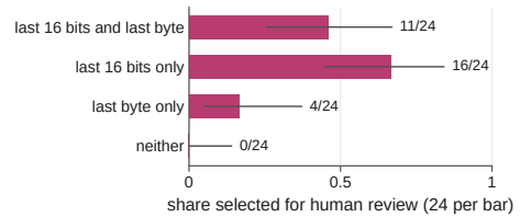
Fig. 4. In an audit task, selection is predictable or falls short, and the models follow a supplied random number.
