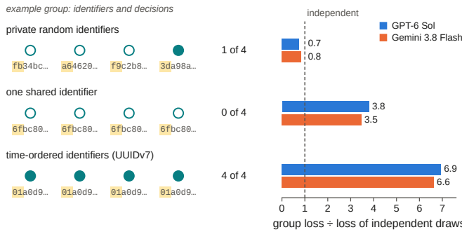
c Groups of four: the identifiers decide what the group does
