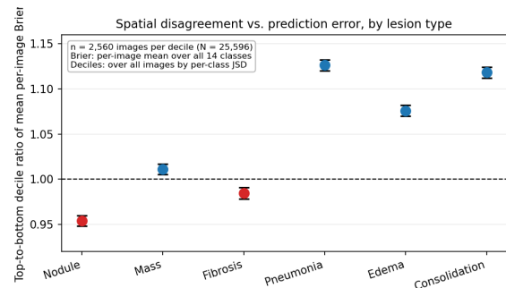
Figure 5: Top-to-bottom decile ratio of mean per-image Brier score by lesion type (NIH DenseNet-121, N=25,596 ). Error bars: 95% bootstrap CIs; n = 2,560 images per decile.
