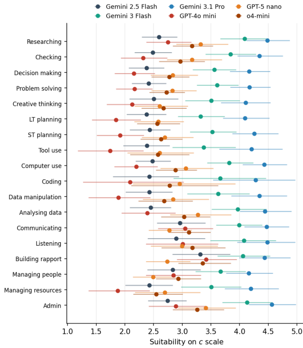
Figure 5: Task suitability of the six AI systems across the 18 work activities on the log-capability ( c = \log \theta ) scale (points: posterior means; bars: 95% credible intervals). Suitability is the importance-weighted power mean of ratio-scale capabilities ( \theta = e^c ), reported as \log S (the weighted mean of c at p = 0 ). Estimates use the full sample ( n = 410 , all domains), with sharpness s = 1 , no column normalisation, and empirical weight uncertainty ( \kappa_t \approx n_t ).
