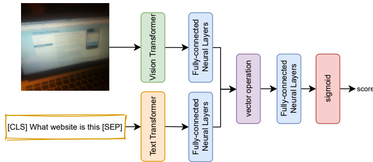
Figure 4: VT-Transformer: combines Vision-Text Transformer features by a vector operation to predict an answerable score in the regression model
