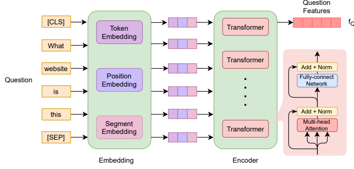
Figure 2: Question Embedding: extracts textual features of words in question by BERT - Text Transformer.
