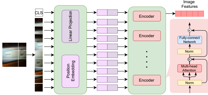
Figure 3: Image Embedding: splits an image into patches and convert it via Linear and Positional Embedding to extract the regional and visual features.
