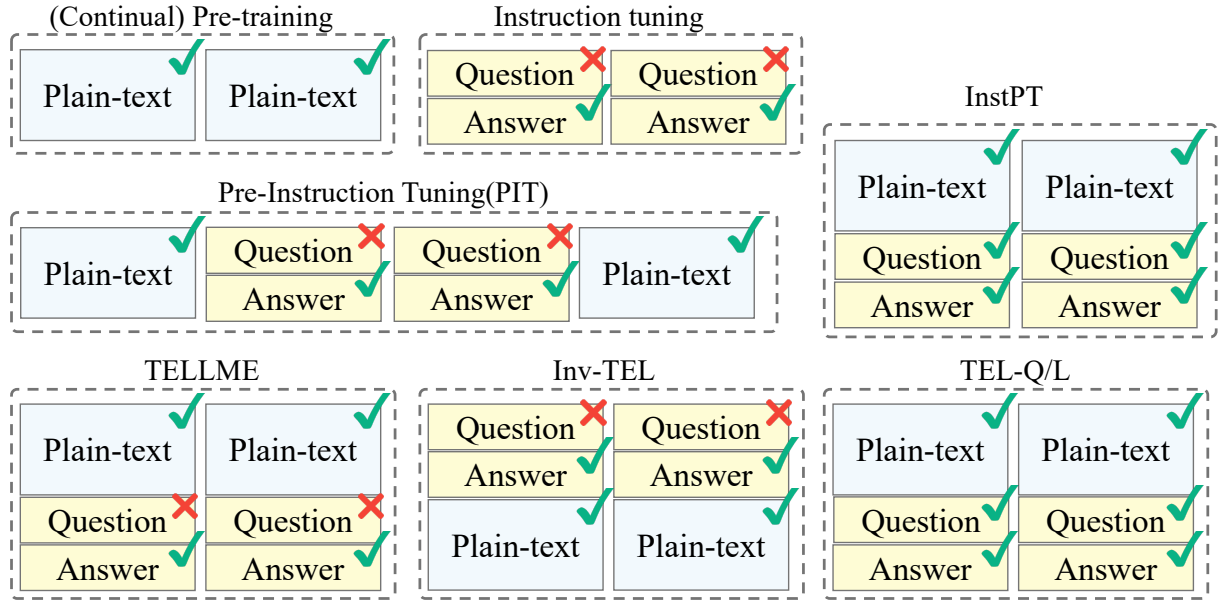
Figure 4: Comparison of data composition and token-level loss masking across training paradigms. Dashed boxes denote individual mini-batches; within each, the vertically stacked panels constitute a single training sequence. (Continual) Pre-training consumes plain text only, applying the objective to every token. Instruction tuning feeds question-answer (QA) pairs but back-propagates loss exclusively on answer tokens. Pre-Instruction Tuning (PIT) interleaves plain text with QA pairs, computing loss on plain-text and answer tokens while masking question tokens. InstPT activates the objective for all tokens in both plain-text and QA examples. Our proposed TELLME keeps PIT’s masking strategy while doubling the proportion of plain-text sequences to reinforce language modeling; its counterpart Inv-TEL inverts the ordering of QA and plain-text segments within each sample. TEL-Q/L serves as a fully supervised upper bound, applying loss to all tokens in both modalities. Green check marks identify tokens whose losses are calculated, whereas red Crossmark denote tokens excluded from loss computation.
