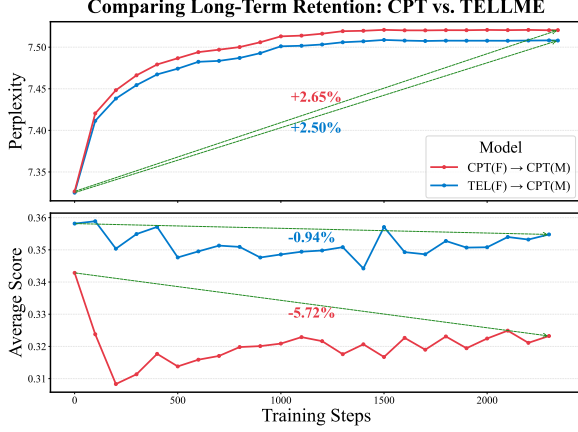
Figure 3: Performance of the finance domain after overwriting with medicine data.
