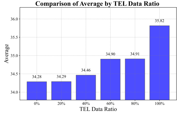
Figure 6: Performance chart illustrating the effect of different ratios of general plain text and the TELLME dataset, using a model trained on finance data. The evaluation is the same financial benchmark used in Table 3
