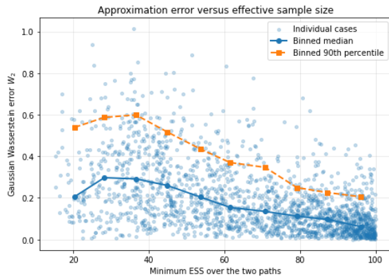
Figure 2: Comparison of the approximation error and the effective sample size. It can be observed that the approximation error tends to decrease when the ESS increases, which indicates that particle degeneracy is one of the main limitations of the current implementation.
