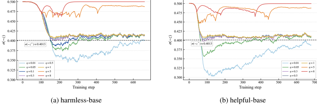
Figure 10: Learning signal \sigma(-z) trajectories of LSC-DPO under different control rates \eta with Llama3-8B on Anthropic-HH subsets. The dashed line marks the target signal \sigma(-z^*) \approx 0.4013 .
