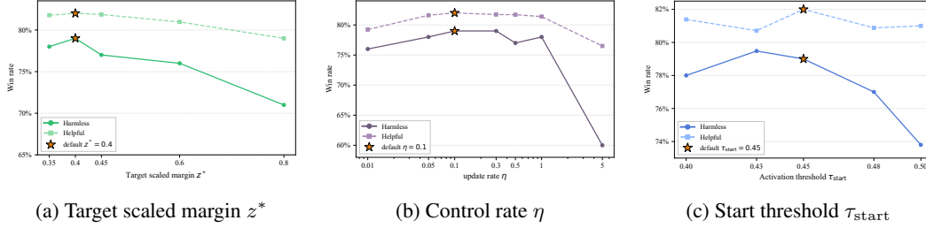
Figure 14: Ablation analysis of key control parameters with Llama3-8B on Anthropic-HH subsets: (a) target scaled margin z^* , (b) control rate \eta , and (c) start threshold \tau_{\text{start}} . The star marks the default setting used in the main experiments.
