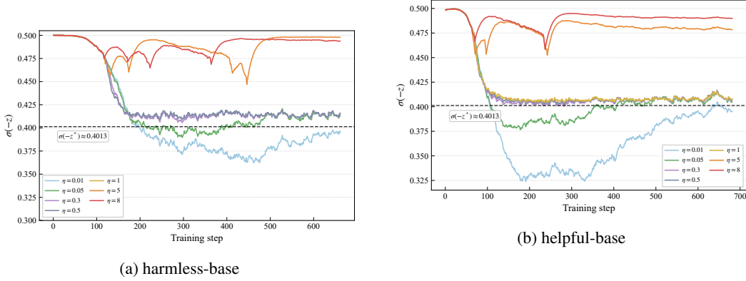
Figure 11: Learning signal \sigma(-z) trajectories of LSC-DPO under different control rates \eta with Qwen3-8B on Anthropic-HH subsets. The dashed line marks the target signal \sigma(-z^*) \approx 0.4013 .
