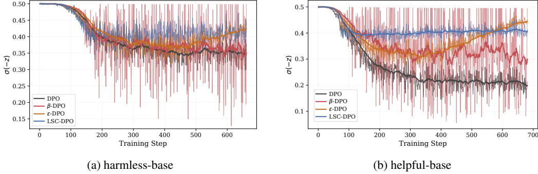
Figure 8: Raw and EMA-smoothed trajectories of the learning signal \sigma(-z) on Anthropic-HH with Qwen3-8B. Faint curves denote raw per-step values, while bold curves denote EMA-smoothed trends.
