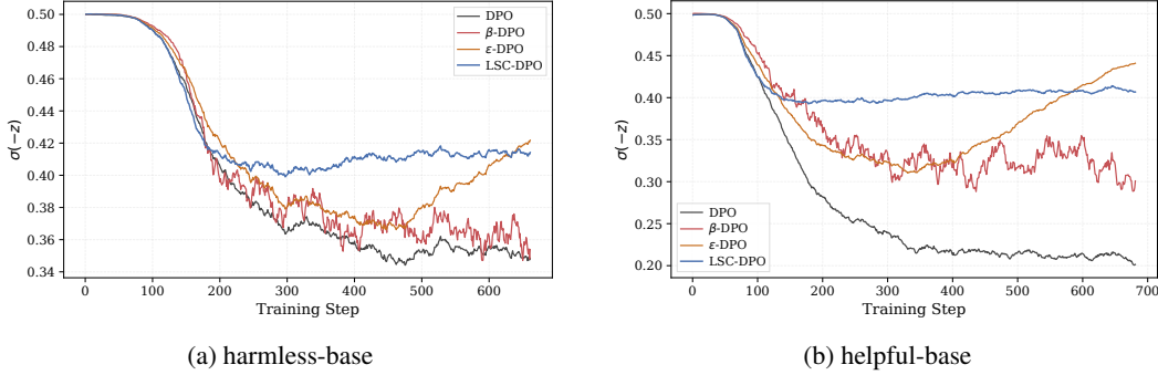
Figure 9: EMA-smoothed trajectories of the learning signal \sigma(-z) on Anthropic-HH with Qwen3-8B.
