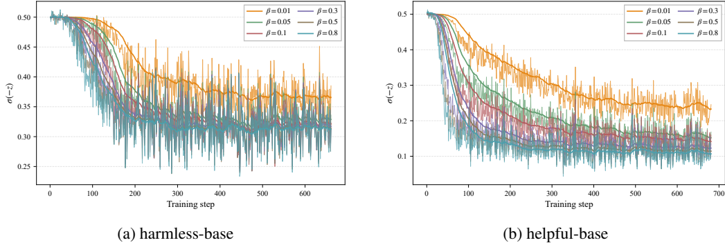
Figure 6: Learning signal under DPO. Raw per-step trajectories of \sigma(-z) are shown for different fixed \beta values on Anthropic-HH: (a) harmless-base and (b) helpful-base.
