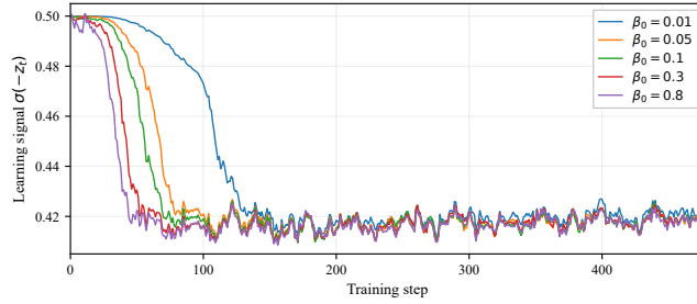
Figure 5: Learning-signal trajectories under different initial \beta_0 . Curves are EMA-smoothed.
