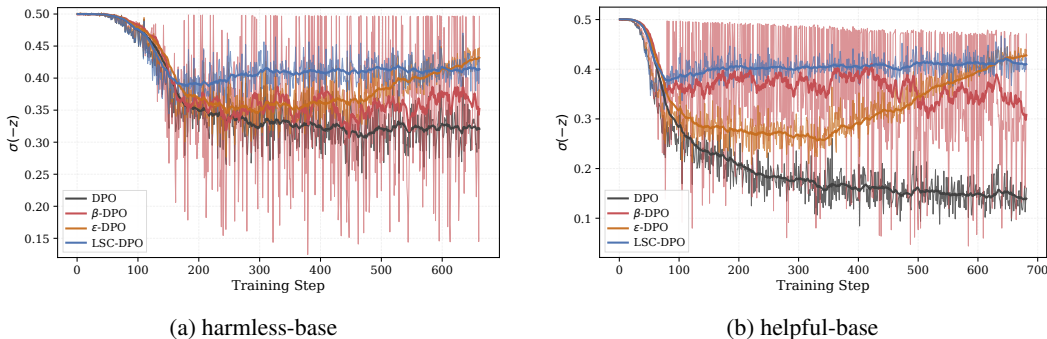
Figure 7: Raw and EMA-smoothed trajectories of the learning signal \sigma(-z) on Anthropic-HH with Llama3-8B. Faint curves show raw per-step values, while bold curves show EMA-smoothed trends.
