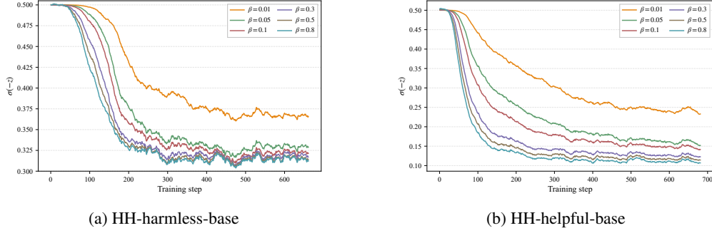
Figure 2: \sigma(-z) under fixed \beta values during DPO training with Llama3-8B on two Anthropic-HH subsets: (a) harmless-base and (b) helpful-base. EMA-smoothed trajectories are shown for readability; raw trajectories are provided in Appendix A.
