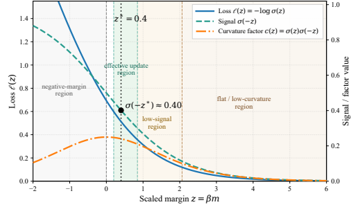
Figure 1: Illustration of the DPO loss geometry as a function of the scaled margin z = \beta m . The learning signal \sigma(-z) and curvature factor c(z) = \sigma(z) \sigma(-z) decrease as z grows.
