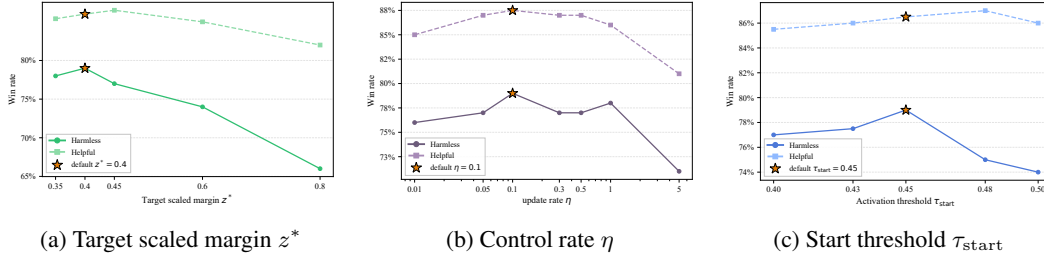
Figure 15: Ablation analysis of key control parameters with Qwen3-8B on Anthropic-HH subsets: (a) target scaled margin z^* , (b) control rate \eta , and (c) start threshold \tau_{\text{start}} . The star marks the default setting used in the main experiments.
