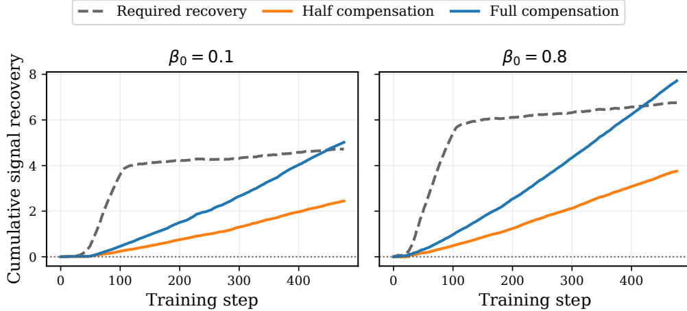
Figure 13: Cumulative learning-signal recovery under half and full signal-budget compensation for \beta_0 = 0.10 and \beta_0 = 0.80 . The dashed curves denote the recovery required to match the anchor run ( \beta_0 = 0.01 ), while the solid curves show the recovery achieved by half and full compensation. Full compensation closely matches or slightly exceeds the required recovery, whereas half compensation recovers approximately half of the deficit.
