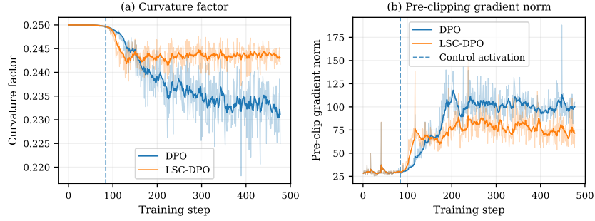
Figure 12: Optimization diagnostics for DPO and LSC-DPO throughout training. Left: curvature factor. Right: pre-clipping gradient norm. The vertical dashed line marks LSC-DPO control activation at step 84.
