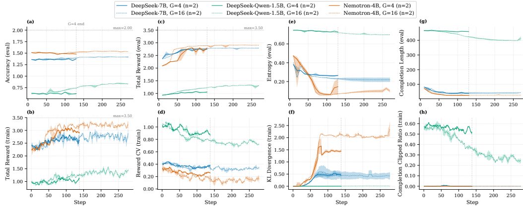
Figure 2: GRPO training dynamics on ARC across models and group sizes ( G \in \{4, 16\} ). Reward and accuracy are largely aligned, with Nemotron-4B performing best, followed by DeepSeek-7B and DeepSeek-R1-Qwen-1.5B. Increasing G yields limited gains for the stronger models but modestly improves DeepSeek-R1-Qwen-1.5B. Diagnostics reveal model-dependent regimes: Nemotron-4B exhibits low entropy with large KL movement, whereas DeepSeek-R1-Qwen-1.5B maintains high entropy, long completions, and persistent clipping.
