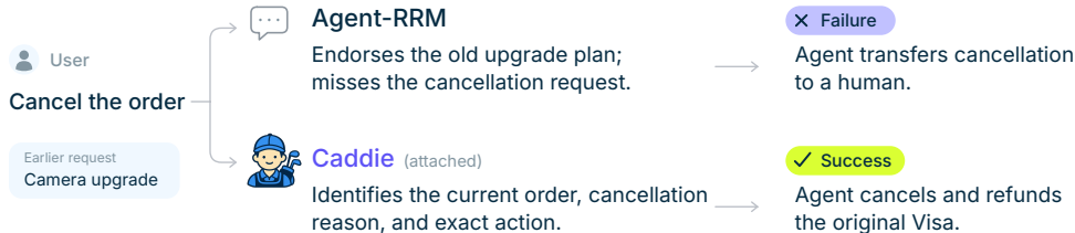
Figure 3. Matched \tau^3 Retail trajectories after the same change in user intent. Each path summarizes the critic advice and the frozen-generator continuation.
