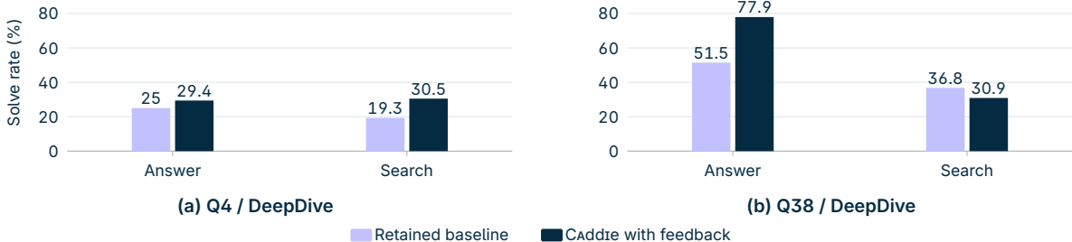
Figure 4. DeepDive solve rate by advice type. Lavender (retained baseline): no-critic rollouts on the tasks where that advice type was given; navy: rollouts that received it.
