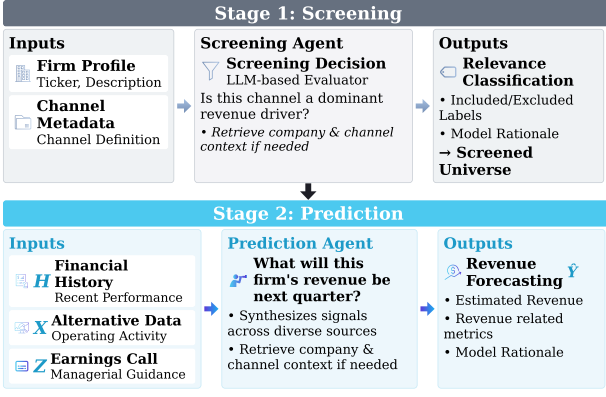
Figure 2: Overview of our framework. Our framework consists of two stages. The screening agent first identifies firm-channel pairs for which an alternative data channel is likely to be informative about the firm’s revenue, filtering out firms for which the channel is unlikely to reflect revenue-generating activity. The prediction agent then forecasts next-quarter revenue by jointly interpreting the firm’s financial history, alternative data, and prior earnings-call transcripts.
