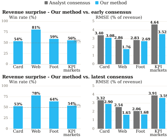
Figure 4: Comparison with analyst consensus on revenue-surprise prediction. We measure Root Mean Square Error (RMSE) and win rate, where win rate denotes the percentage of events for which prediction of our method is closer to the realized revenue surprise than the consensus estimate. The top row uses the early consensus snapshot (available shortly after quarter end), while the bottom row uses the latest consensus immediately before the earnings.
