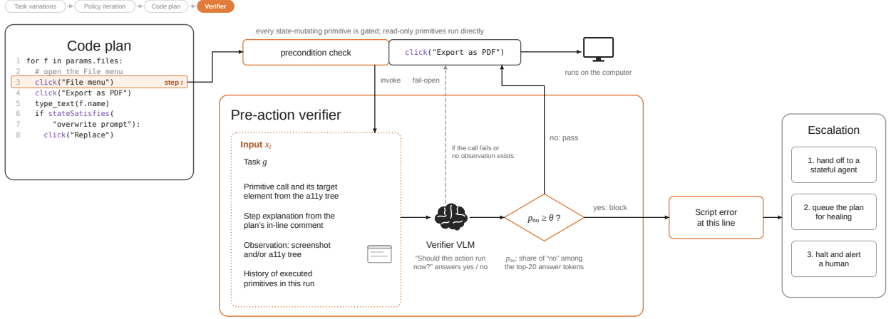
Figure 6 | A learned binary-output pre-action verifier V runs before every state-mutating primitive during policy deployment. Reusing the plan’s most recent stashed screenshot and accessibility tree, V emits top-20 answer-token logprobs; the yes/no log-mass is renormalized to p_{no} and the action is blocked iff p_{no} \geq \theta . A block raises a script-level error at the offending line, triggering the fallback hierarchy (agent hand-off, code repair, halt).
