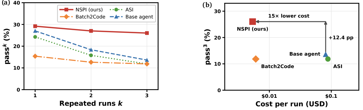
Figure 3 | Repeated-execution reliability and execution cost on ScienceBoard with GPT-5.6-Terra. (a) NSPI maintains high \text{Pass}^k as k increases, while agent-based baselines degrade more sharply and the Batch2Code conversion-only baseline remains consistent but less accurate. (b) NSPI achieves highest \text{Pass}^3 with efficient per-run execution cost over baselines. Policy-construction cost is analyzed separately in Section 4.4.
