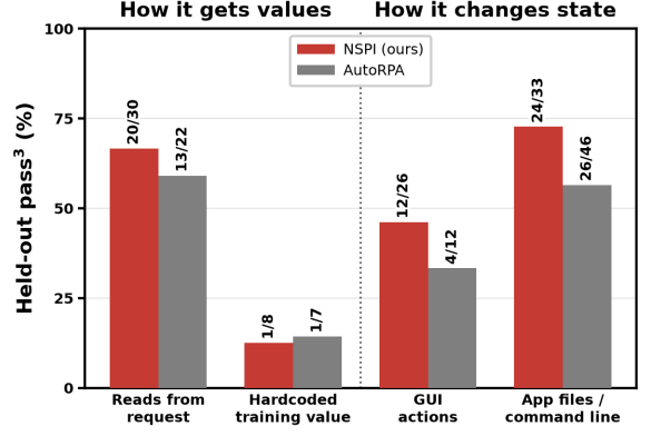
Figure 5 | Policy structures associated with successful reuse across workflow instances. Labels show the number of successful policies out of total applicable policies.
