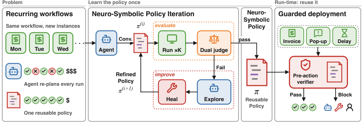
Figure 1 | Recurring computer workflows require reliable repeated execution with generalizability at low cost. In Neuro-Symbolic Policy Iteration : a baseline agent’s exploration seeds an initial neuro-symbolic policy, which preserves the workflow’s stable structure in code while retaining neural primitives for observation-dependent decisions. Our framework iteratively executes, evaluates, diagnoses, and improves the policy with additional agent continuation. The resulting policy is reused across workflows and guarded with pre-action verifiers during run-time deployment.
