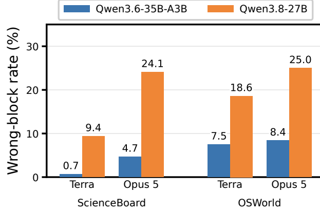
Figure 8 | Pre-action verifier error rates at \theta = 0.78 . Rollout-level wrong-block rate on correct policies, by environment, base model used for initial trajectory seed, and verifier model.
