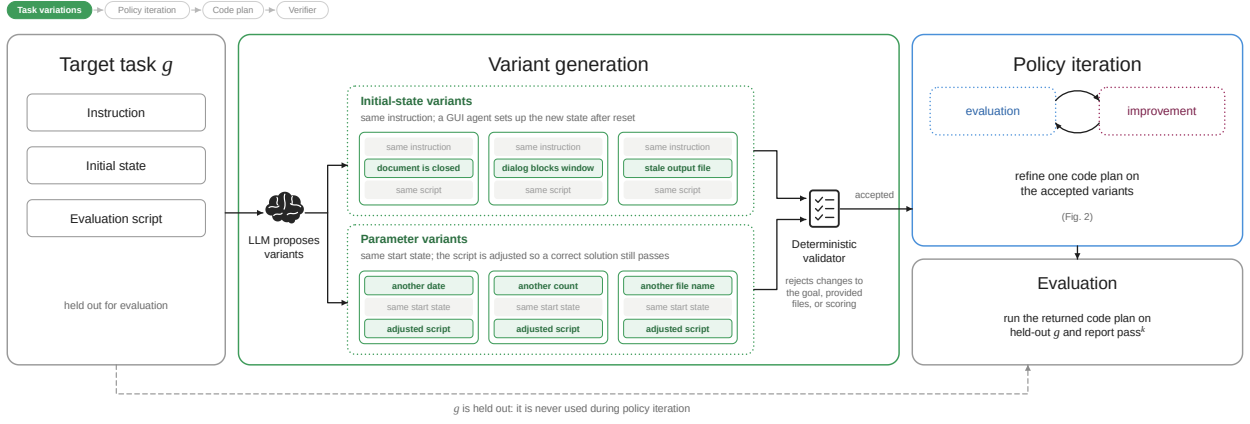
Figure 7 | Given an original target task and environment configuration (initial state and evaluation script), we call an LLM to generate synthetic task variants that differ in the initial state and task parameters
