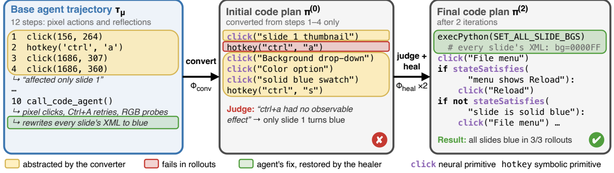
Figure 2 | Example of NSPI converting agent trajectory into a reusable, abstracted neuro-symbolic policy and using judge feedback to identify and heal failures. The resulting policy combines state-dependent control flow, task parameters in code, and neural primitives for grounding (Section 4.1).
