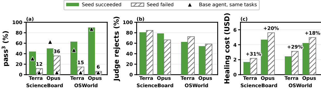
Figure 4 | NSPI can recover reliable policies even from unsuccessful seed trajectories, but at higher cost. (a) \text{Pass}^3 , with base-agent performance on the same tasks. (b) Judge rejection rate during policy iteration. (c) One-time healing cost with the relative increase when initialization uses failed seeds.
