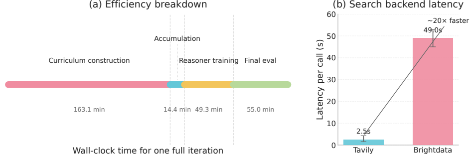
Figure 4: (a) Wall-time breakdown for a full MedZERO self-evolution iteration. (b) Web search latency per call (end-to-end wall time, measured in the same execution environment across 5 consecutive calls).
