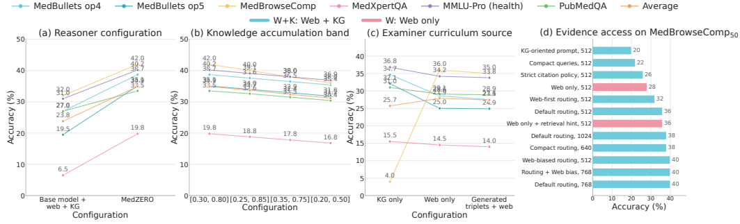
Figure 3: Component analysis across (a) Reasoner configuration, (b) ephemeral-to-persistent accumulation band, and (c) Examiner curriculum source. (d) MedBrowseComp50 evidence-access ablations. W+K = web_search+kg_search; W = Web only.
